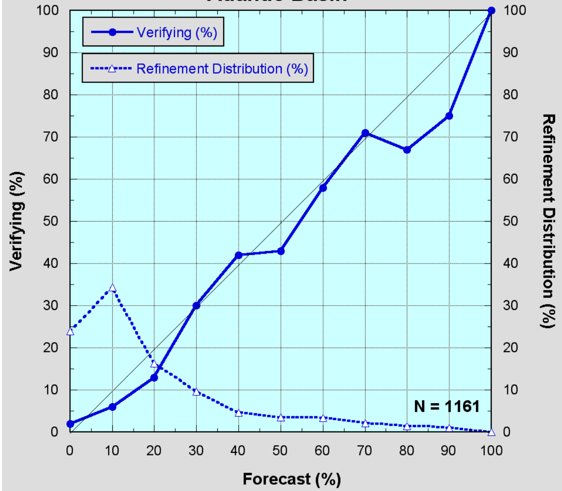
Figure 15a. Reliability diagram for experimental Atlantic probabilistic tropical cyclogenesis forecasts for the period 2007-9. The solid blue line indicates the relationship between the forecast and verifying genesis percentages, with perfect reliability indicated by the thin diagonal black line. The dashed blue line indicates how the forecasts were distributed among the possible forecast values.
