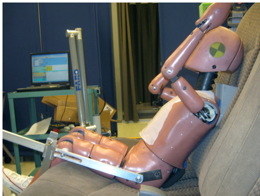
Figure 33. Propping ATD head off the seat back
