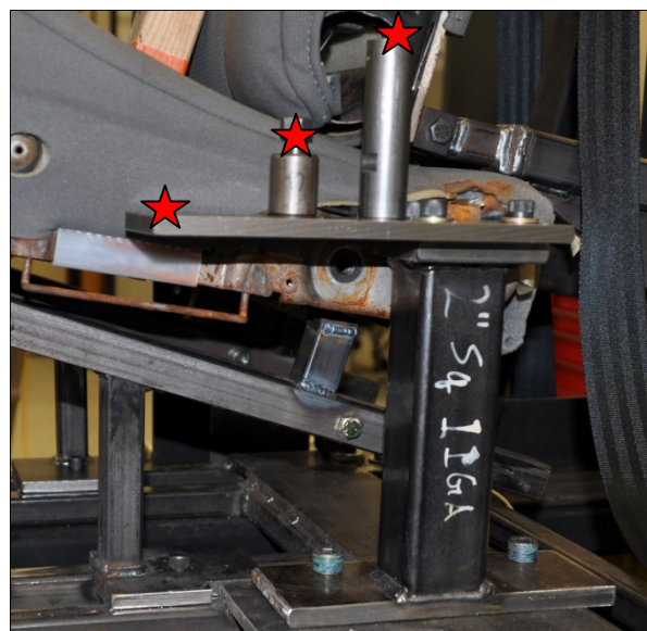
Figure 4. Close-up of inboard anchorage hardware that provides lap belt angles of 23°, 50°, and 75°. (Stars indicate anchorage bolt locations).
