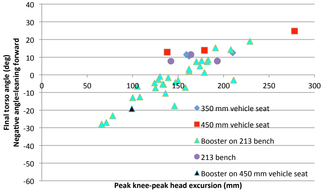
Figure 18. Kinematic results of the 6YO ATD from current study compared to prior testing on the 213 bench with and without booster seats.
