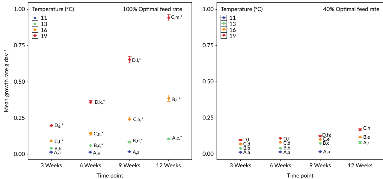
FIGURE 1 Mean \pm S.E. mass growth rates ( \text{g day}^{-1} ) for green sturgeon Acipenser medirostris reared at different temperatures and food availabilities. Capital letters indicate significant differences among temperature treatments at one time point. Lowercase letters indicate significant differences over time within each treatment. Asterisks indicate significant differences between food availability treatments within a temperature and time point. Timepoints at 3, 6, 9, and 12 weeks correspond to 59, 80, 101, and 102 days post hatch (dph), respectively
