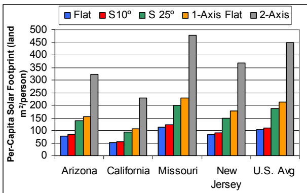
Figure 3. Solar PV Per Capital Land-use Requirement for Four States.
