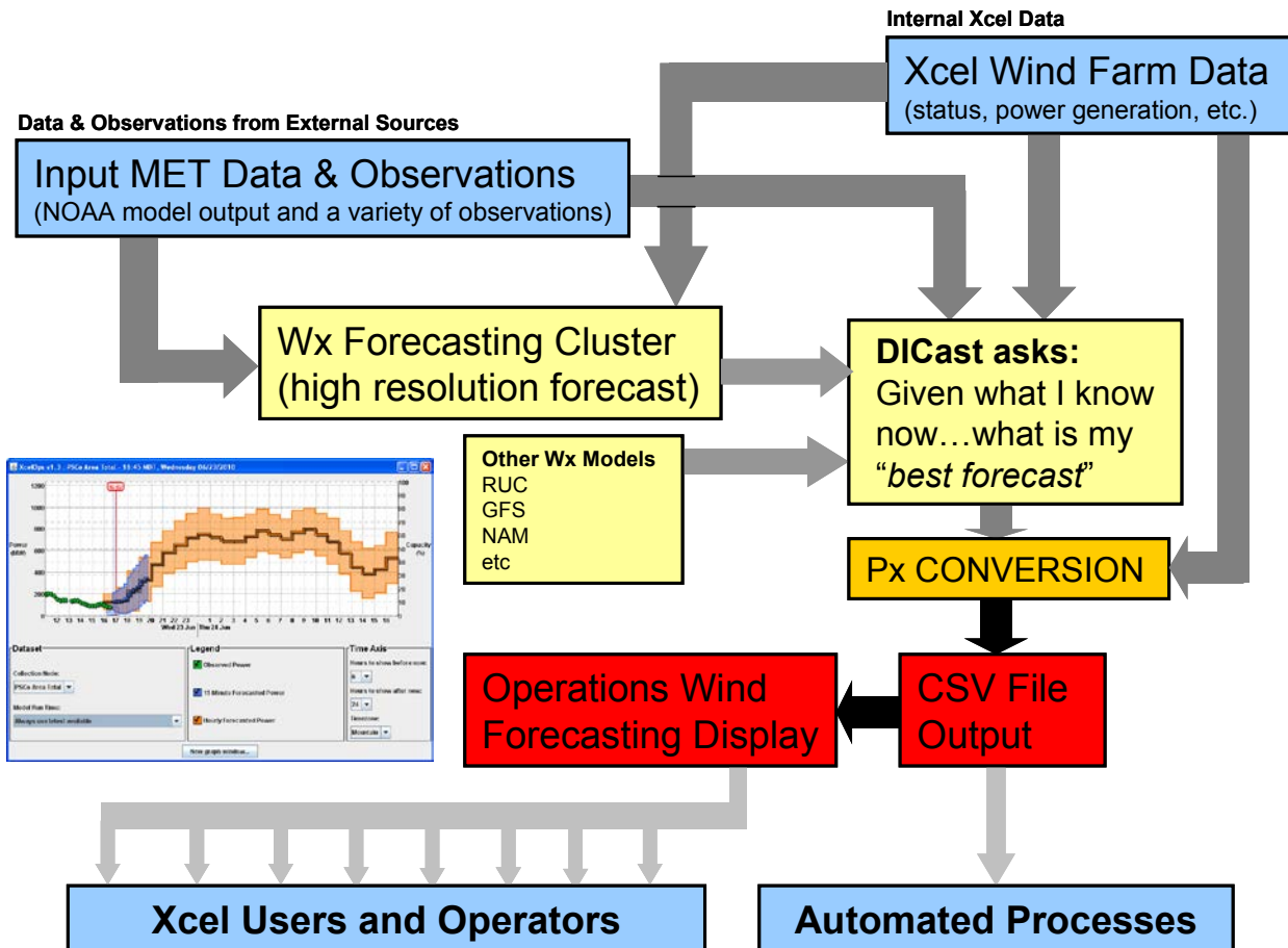
Figure 1 – Xcel Energy Wind Forecasting System.
