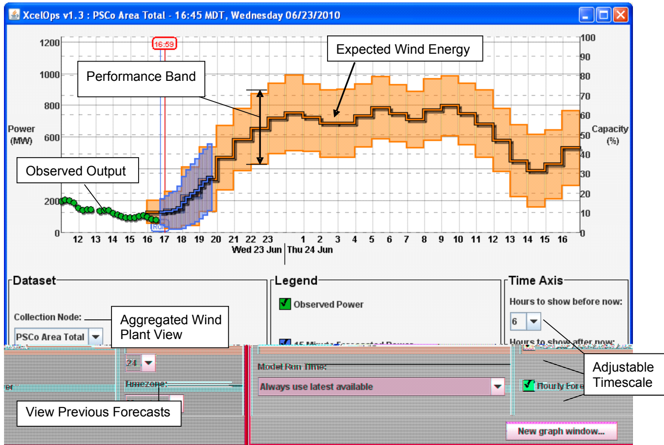
Figure 12 – Operator’s GUI.
