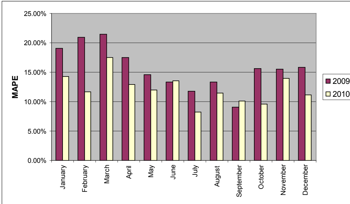
Figure 14 – NSP monthly day-ahead forecast error.
