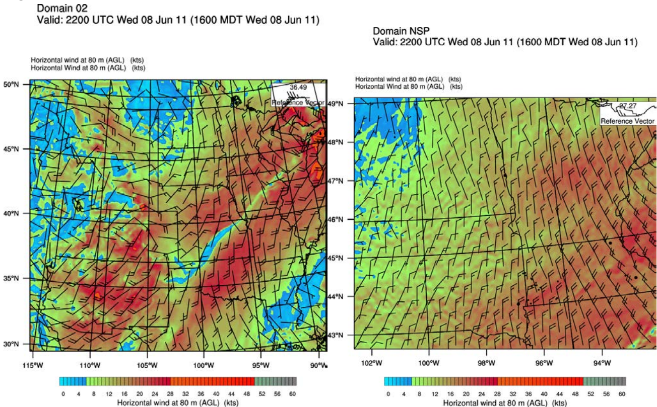
Figure 11 – Wind Speeds at 80m; 10-km and 3-km Domain.
