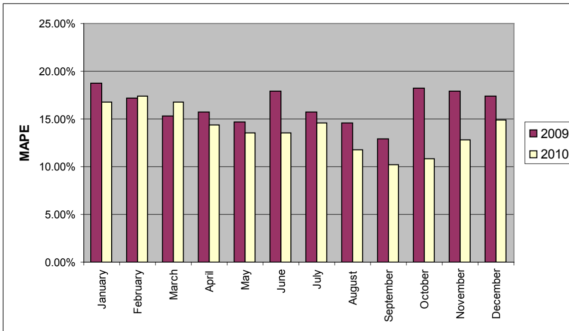
Figure 15 – SPS monthly day-ahead forecast error.
