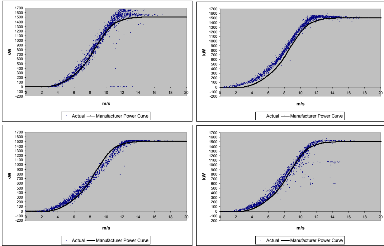
Figure 7 – Same Turbine Type at Four Different Wind Plants.
