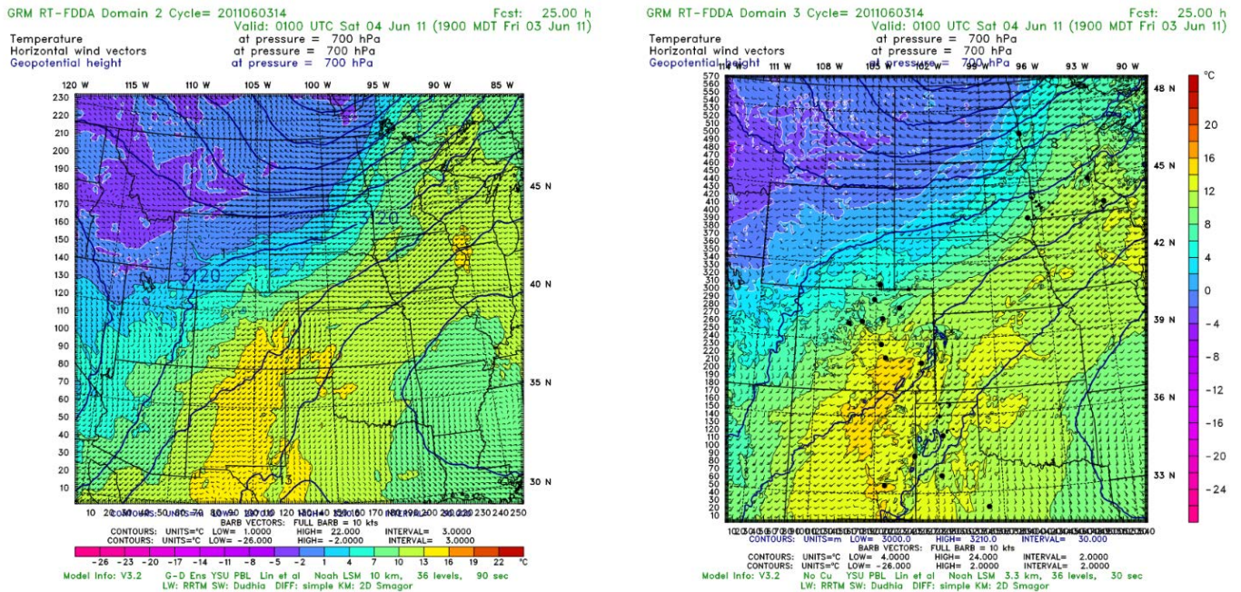
Figure 10 – 700mb Height Temperature and Wind Vectors; 10-km and 3-km Domain; 25-hr Forecast.
