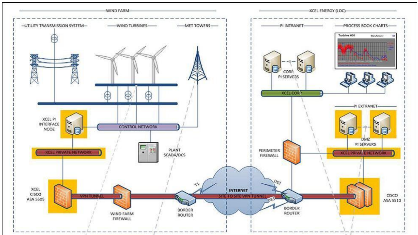
Figure 3 – Schematic of Turbine-Level Data Collection.
