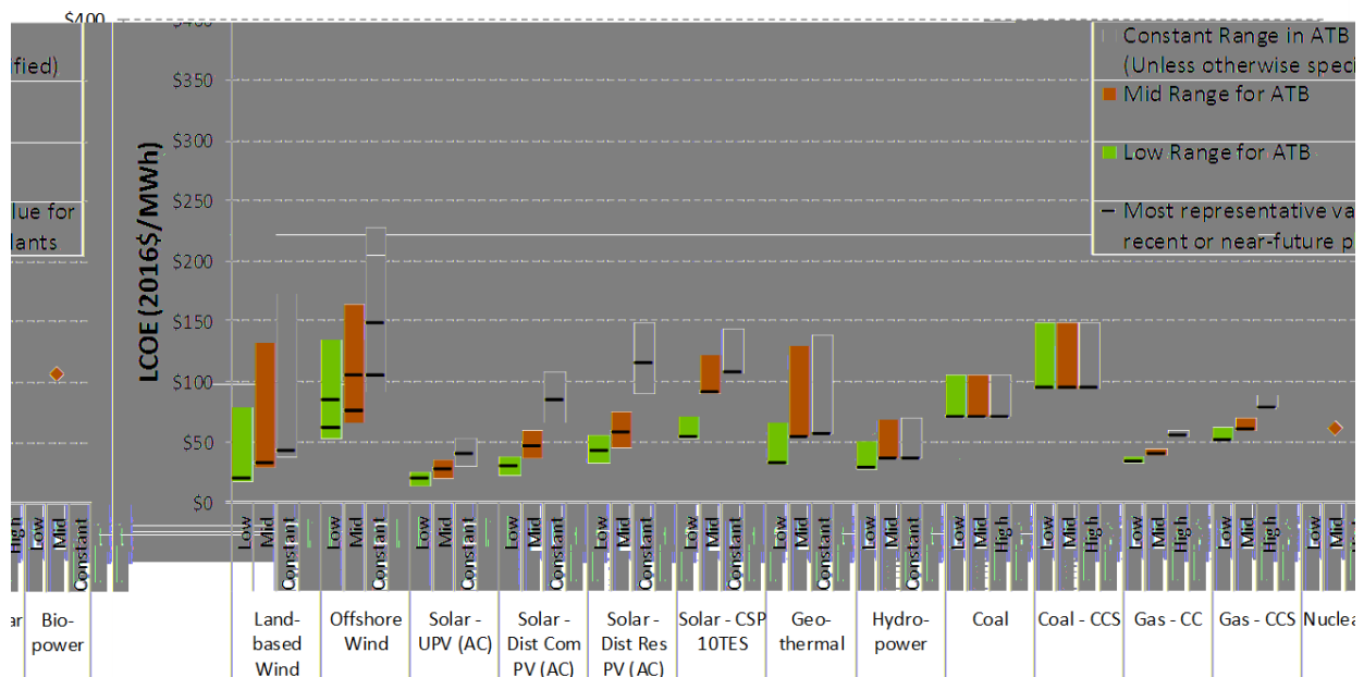
2018 ATB LCOE range by technology for 2030 based on R&D financial assumptions
