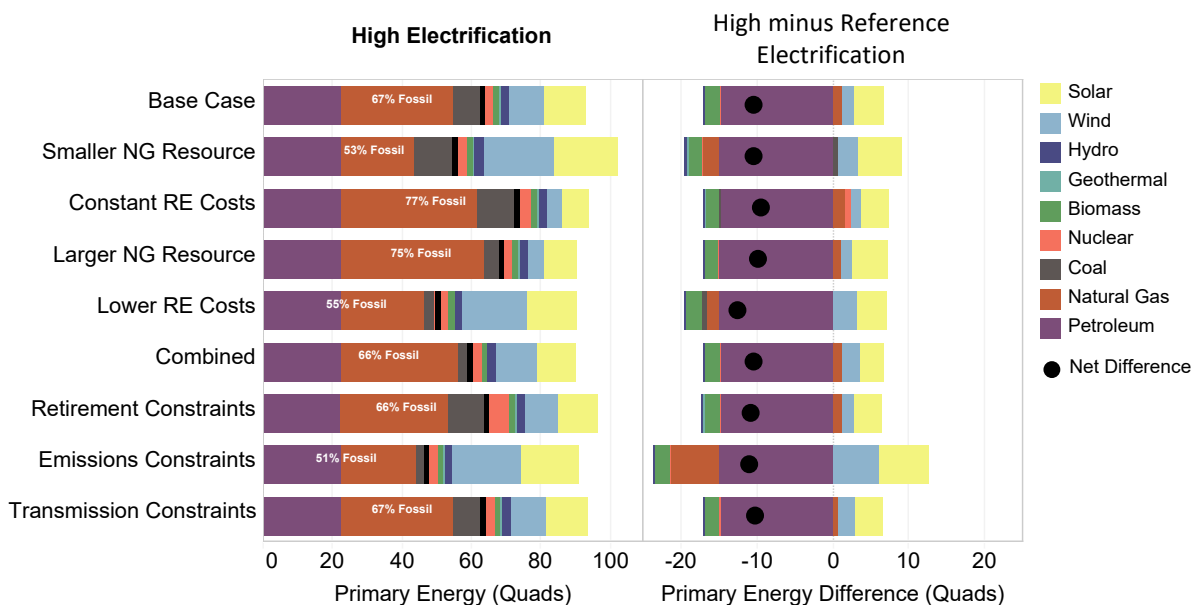
Figure 26. Cumulative (left) and incremental (right) effects of High electrification on 2050 primary energy consumption estimates across all fuel, technology, and system constraint sensitivities
