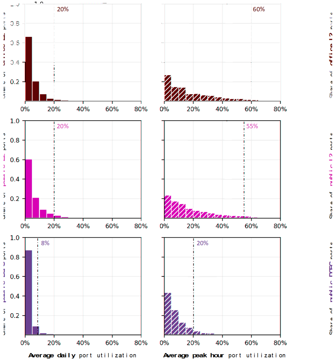
Figure 19. Distribution of average daily port utilization and average peak hour port utilization by location and EVSE type.
