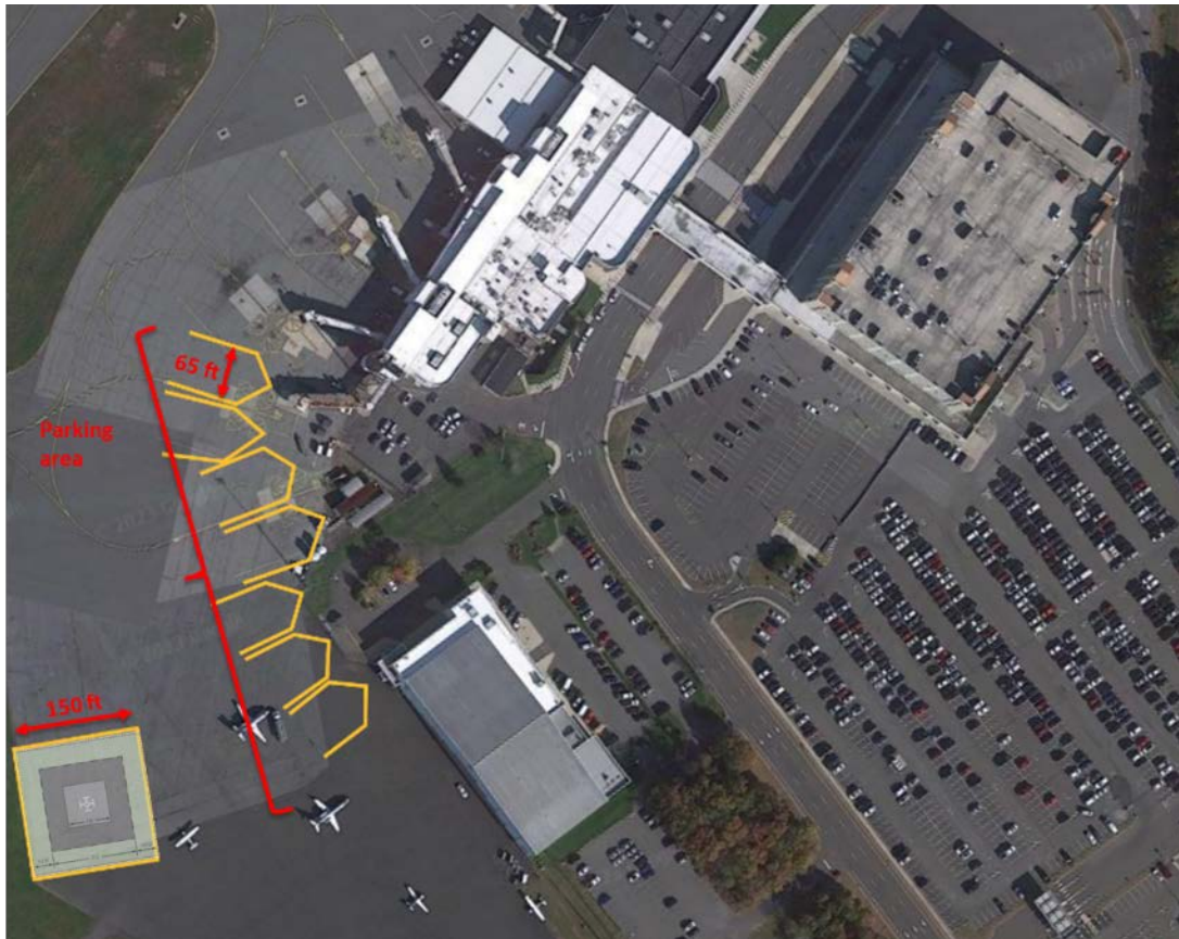
Figure 30. Example eVTOL Parking and Takeoff and Landing Area at ACY.
