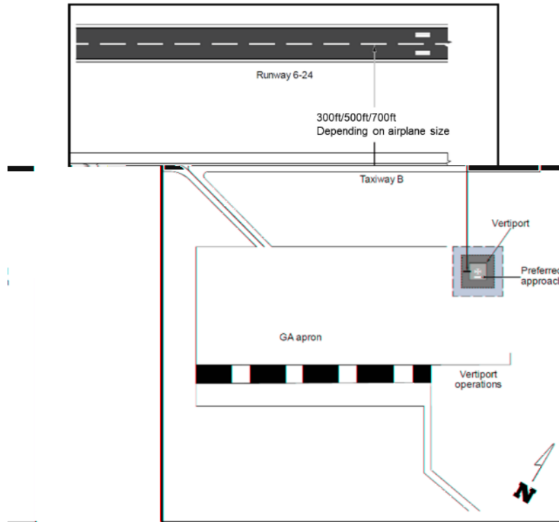
Figure 10. Example of an On-Airport Vertiport (FAA 2022)
