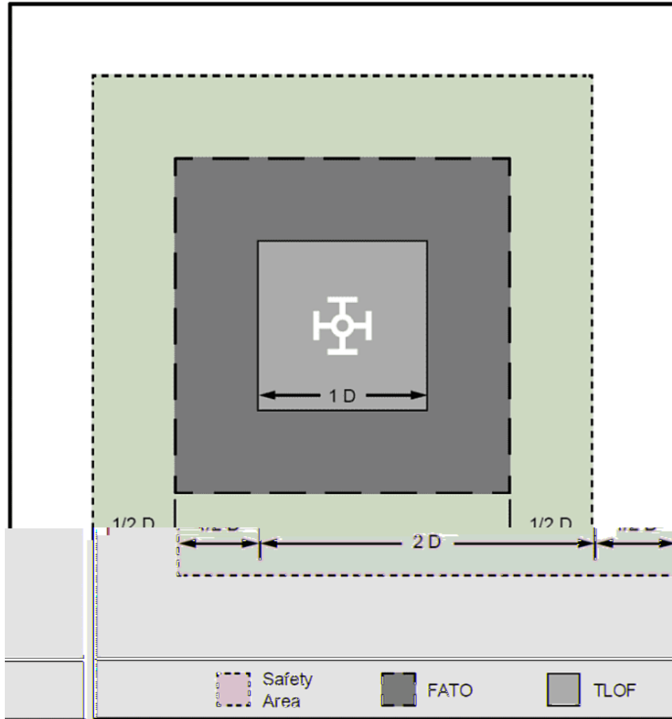
Figure 6. FAA Vertiport Dimensions (FAA 2022)
