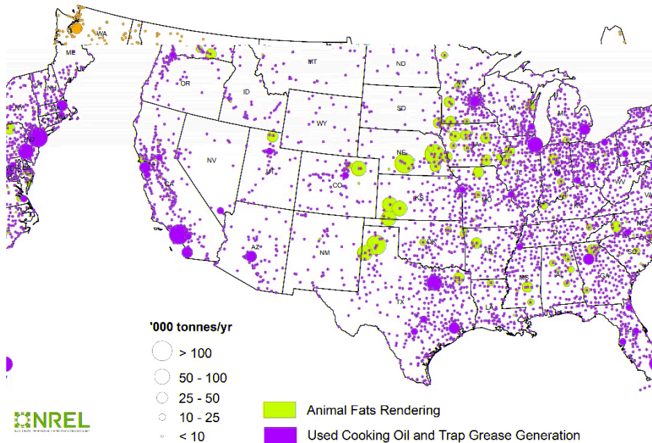
Figure 3. FOG production in the U.S. (2017).
