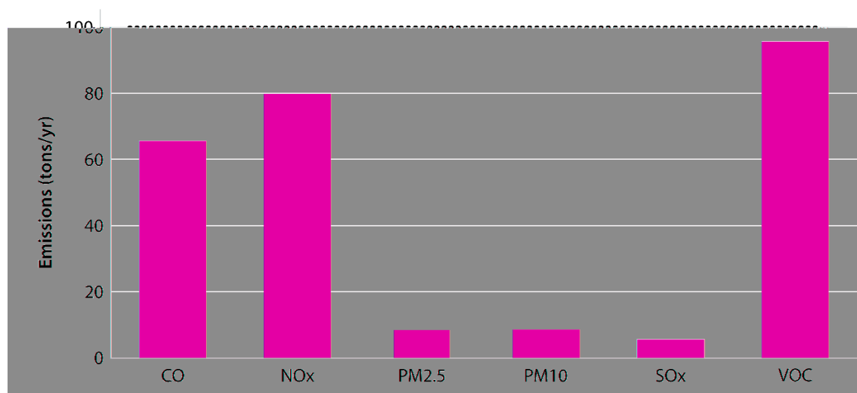
Figure F-2. Montana Renewables LLC criteria pollutants at about 173 MGPY barrels/day of feedstock capacity. Dotted line represents the major source thresholds applicable to Montana Renewables.
