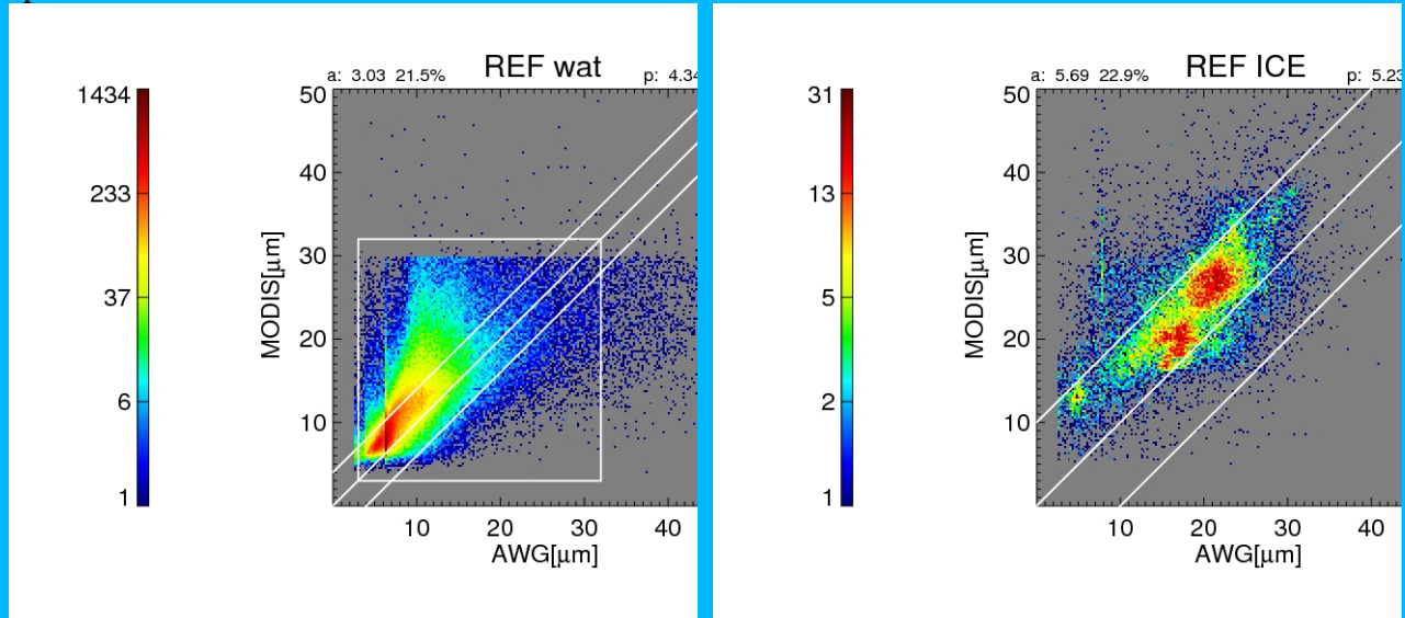
Figure 25 Comparison of Cloud Particle Size for Days 230-239 in 2006 derived from MODIS (MYD06 and MOD06) products and from DCOMP algorithm. Left image shows results for water phase, right image for ice phase. Accuracy and precision of the comparison are shown in the figures. Specs ranges are added as white lines in the figures.
