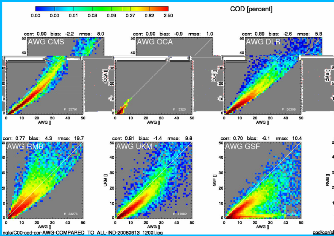
Figure 21 Comparison of DCOMP-COD Ice phase with six other groups.
