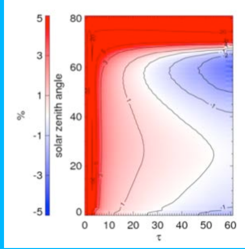
Figure 10 Potential error in percent if Rayleigh correction is not applied as a function of \tau_c and solar zenith angle. Observation angle is 43 degrees and effective radius is 8 \mu m .
