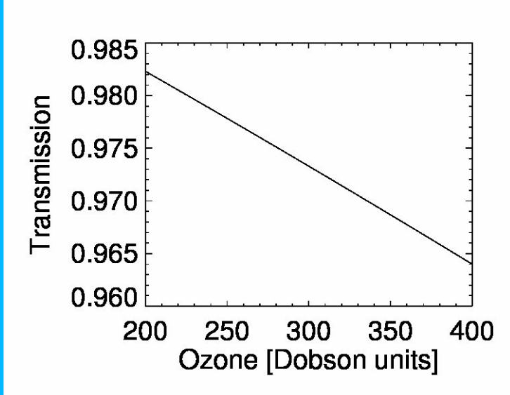
Figure 12 Ozone transmission as a function of absorber amount
