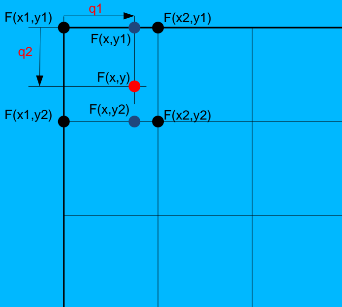
Figure 9 Pictorial depiction of LUT linear interpolation in both one and two dimensions.
