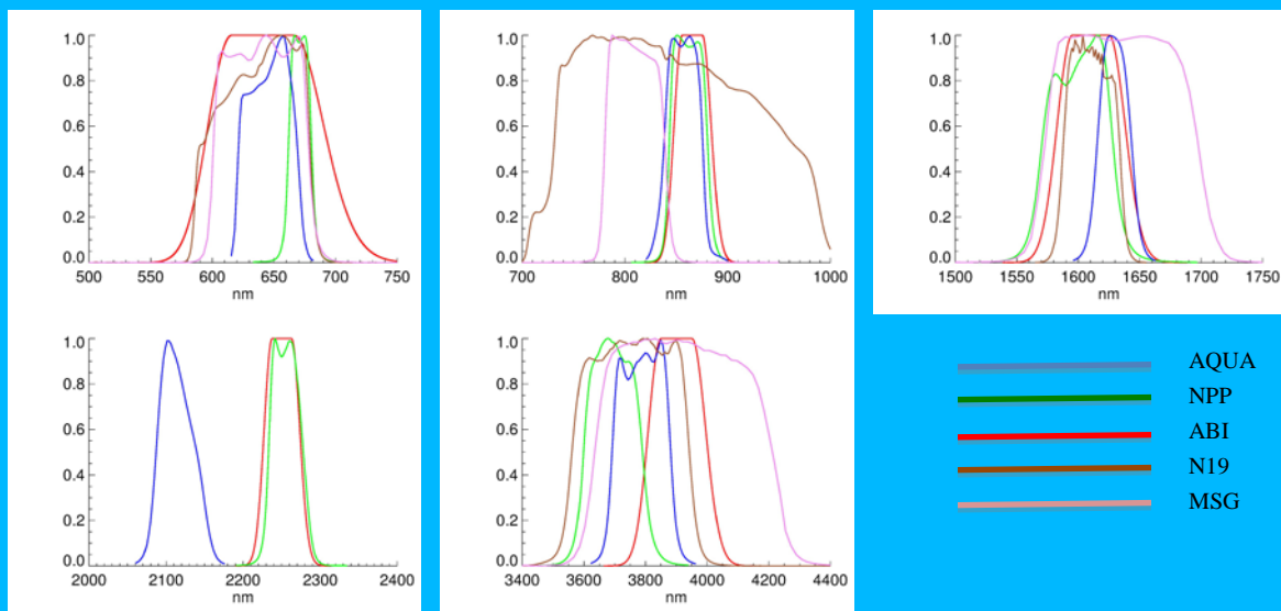
Figure 1 Channel response functions for DCOMP channels 1-5 for five sensors.
