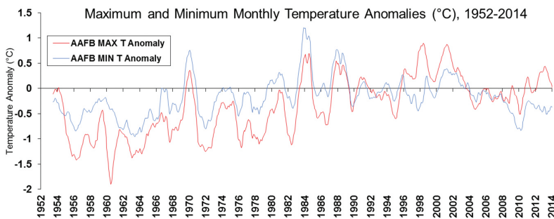
Figure 2. Maximum and minimum monthly temperature anomalies as a 12-month moving average at Andersen Air Force Base (AAFB). Values are expressed as departures from the 1981–2010 base period 3 .
