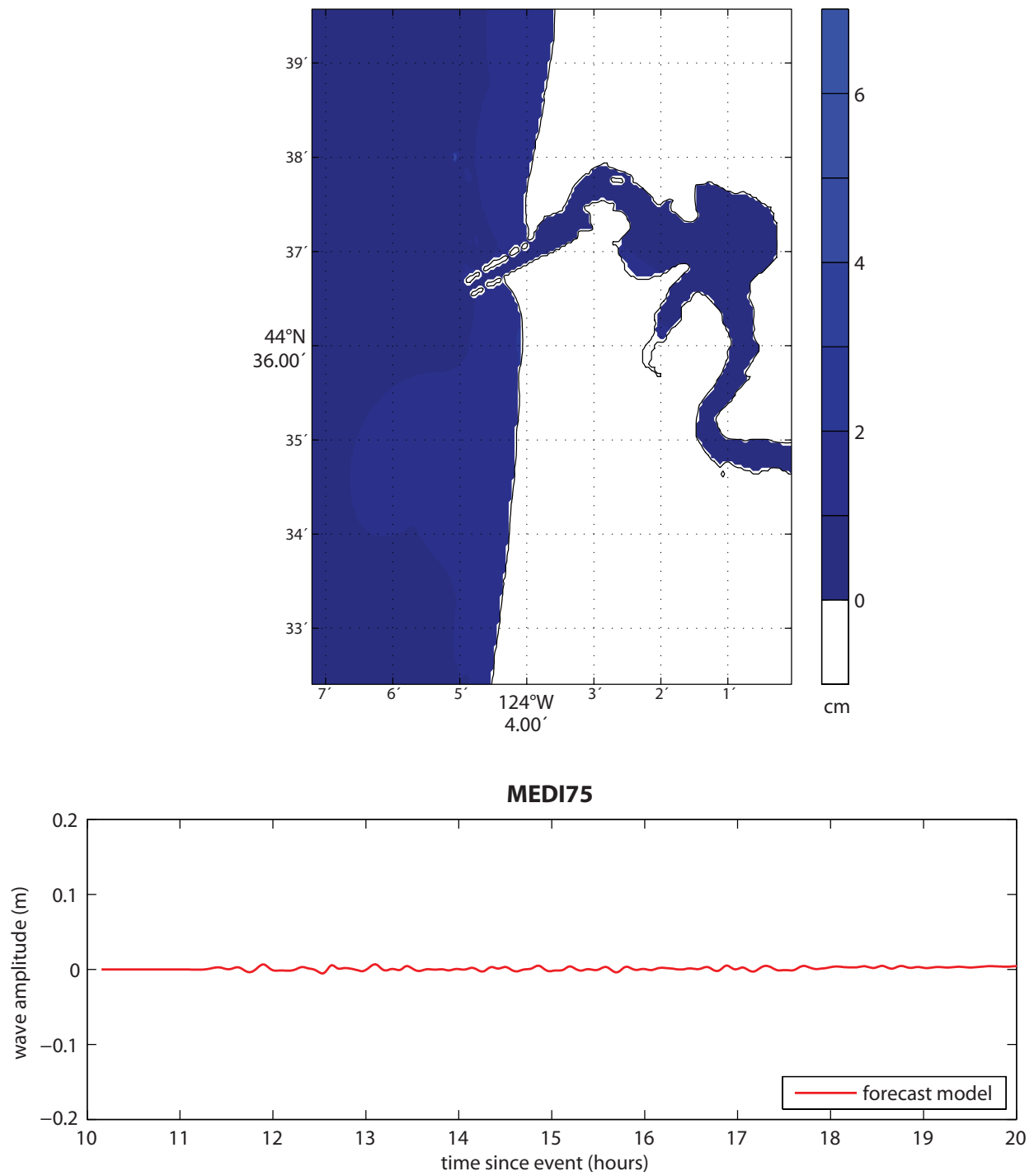
Figure 40: Results from the forecast model for the MEDI7.5 synthetic event forced by a Mw 7.5 rupture of NTSZ B36. The upper panel shows the map of predicted maximum wave height in the Newport C grid and the lower panel shows the time series of wave amplitude at the tide gauge location.
