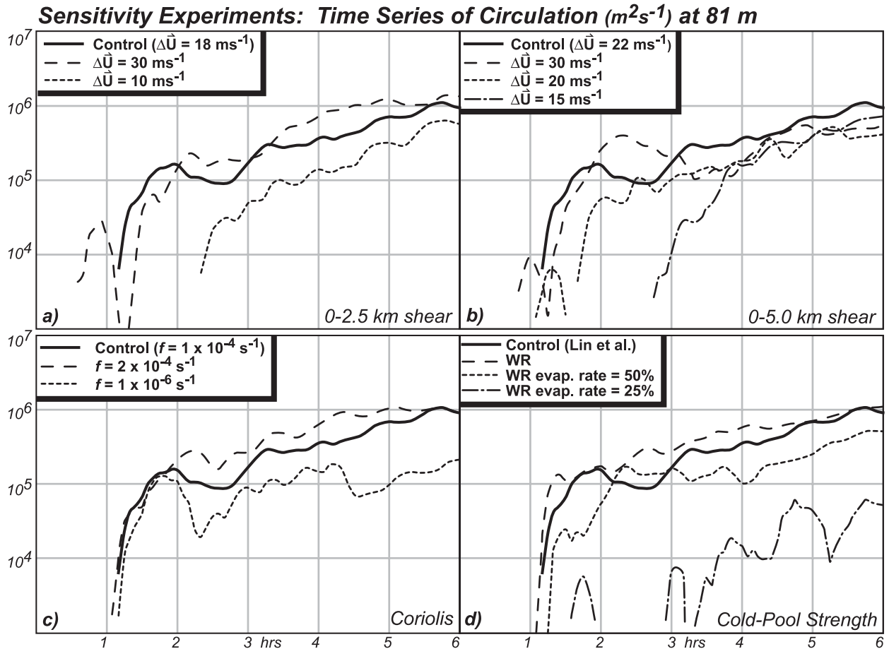
FIG. 5. Time series of circulation ( m^2 s^{-1} ) calculated at the lowest model grid level (81 m) for the different sensitivity experiments. The sensitivity experiments include (a) low-level shear, (b) deep shear, (c) Coriolis forcing, and (d) cold-pool strength. The thick solid line in (a)–(d) represents the control run.
