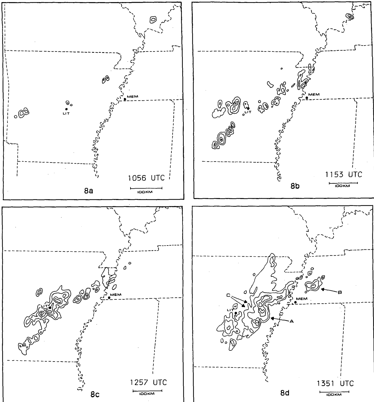
FIG. 8. (a) Radar reflectivity pattern at 1056 UTC 9 April 1991 from the PPI presentation of the Memphis, Tennessee, WSR-74S radar. Contours are NWS VIP levels. Elevation angle 0.5^\circ . Shows isolated convection developing along cold front (see Fig. 3b). (b) Same as (a) except at 1153 UTC: Convection beginning to intensify and move ahead of cold front. (c) Same as (a) except at 1257 UTC. Convection continues to intensify ahead of the cold front. (d) Same as (a) except at 1351 UTC. Eastward bulge at A may indicate echo has started to "bow" outward. (e) Same as (a) except at 1450 UTC. Arrow at A points to major WEC. Damaging winds (measured to 34 \text{ m s}^{-1} ) are occurring at Memphis, Tennessee (MEM), beneath the tight reflectivity gradient just east of the WEC. (f) Composite radar presentation at 1621 UTC, derived from information from the WSR-74S radar at Memphis and the WSR-57 radar at Nashville (BNA). Contours are NWS VIP levels. Arrows at A point to WECs. Stippled area shows a rain-free area immediately to the rear of the bowed-out part of the squall line. (g) Radar reflectivity pattern at 1708 UTC 9 April 1991 from the PPI presentation of the Nashville WSR-57 radar. Contours are NWS VIP levels. Elevation angle 0.5^\circ . Arrow at A points to center of rotation seen in looped radar data. (h) Same as (g) except at 1735 UTC. Arrow at A points to possible rotation center. (i) Same as (g) except at 1833 UTC. Arrows at A point to some WECs. The stippled area (B-C-D) highlights the rain-free area between the squall line and the trailing precipitation. Arrow at E points to center of possible rotation. (j) Same as (g) except at 1917 UTC.
