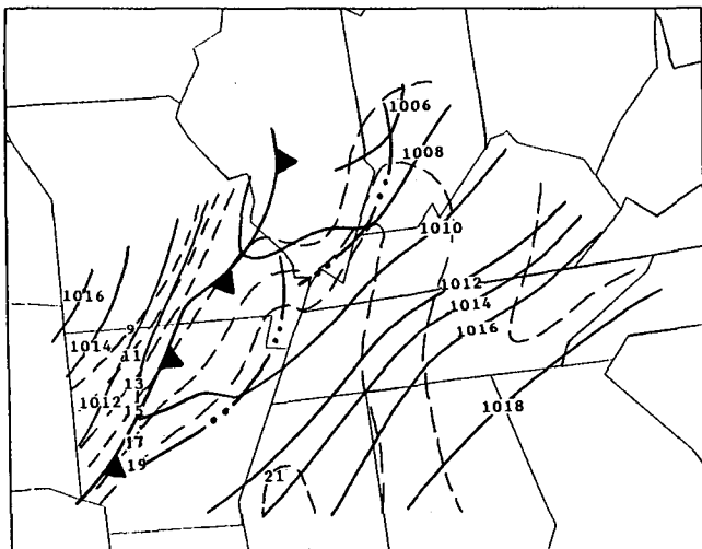
FIG. 3. (a) 1200 UTC 9 April 1991 850-mb analysis. Solid lines are isoheights (meters), light dashed lines are isotherms ( ^{\circ}\text{C} ), heavy dashed lines are trough axes. Stippled areas show locations of T_d > 9^{\circ}\text{C} . (b) 1200 UTC 9 April 1991 surface analysis. Solid lines are isobars, drawn every 2 mb. Dashed lines are isodrotherms, drawn every 2^{\circ}\text{C} . Dash-double-dot-dash lines mark surface outflow boundary locations.
