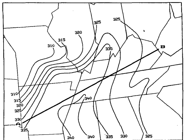
FIG. 5. 1200 UTC 9 April 1991 surface equivalent potential temperature \theta_e . Line connecting points A and B is near main damage path during derecho development and early evolution.
