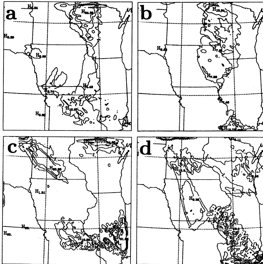
FIG. 12. Same as in Fig. 11, but using the KF convective scheme. (a), (c) Output from the run initialized with Eta output and (b), (d) initialized from AVN output. Contours are the same as in Fig. 5.
