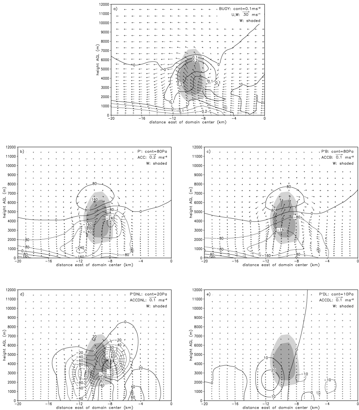
FIG. 20. Same as Fig. 14, but for simulation FFTS (MOIST) at 833 s, with W shaded at 5 and 10 m s -1 .
