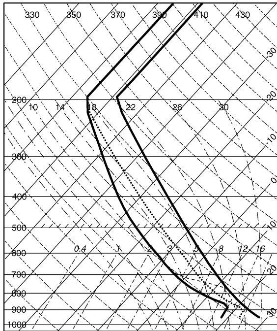
FIG. 10. Skew T -log p diagram of the mean MCS sounding used in this study, along with two modifications (described in the text). The control, mean MCS sounding (CTRL) is plotted with thick solid curves. The humidity profile for the moistened sounding (MOIST, with q_{\text{afc}} = 0.22 and r_{\text{min}} = 0.65 ) is plotted with a medium-weight dotted curve. The humidity profile for the deepened \theta_e maximum sounding (DEEP) is plotted with a thin-dashed line. Bulk thermodynamic variables for the CTRL sounding are given in Table 1.
