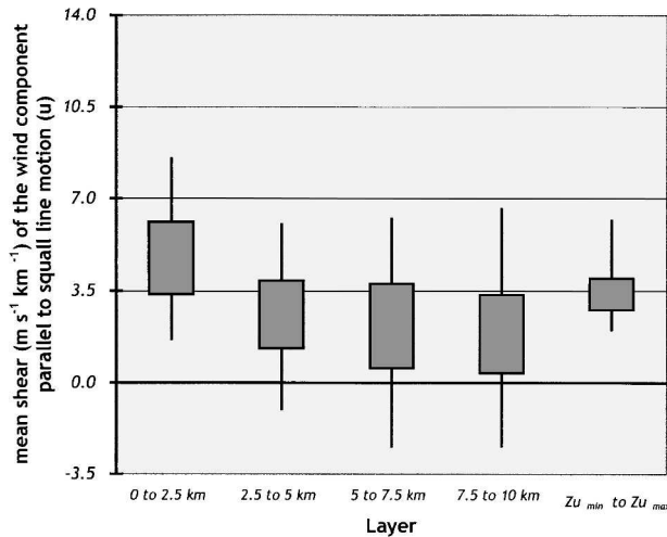
FIG. 2. The range of the mean shear ( \text{m s}^{-1} \text{km}^{-1} ) of the wind component parallel to squall-line motion ( u ) in various layers. The mean shear for each sounding is calculated by the difference in u between the two levels. The depth “ Zu_{\min} to Zu_{\max} ” refers to the layer that is bounded by the minimum and maximum u for each sounding, and is usually 8–12 km deep. This depth is used to calculate the deep layer shear values depicted in Fig. 1. Boxes denote the 50% of the distribution between the 25th and 75th percentiles. The vertical lines extend to the 5th and 95th percentiles.
