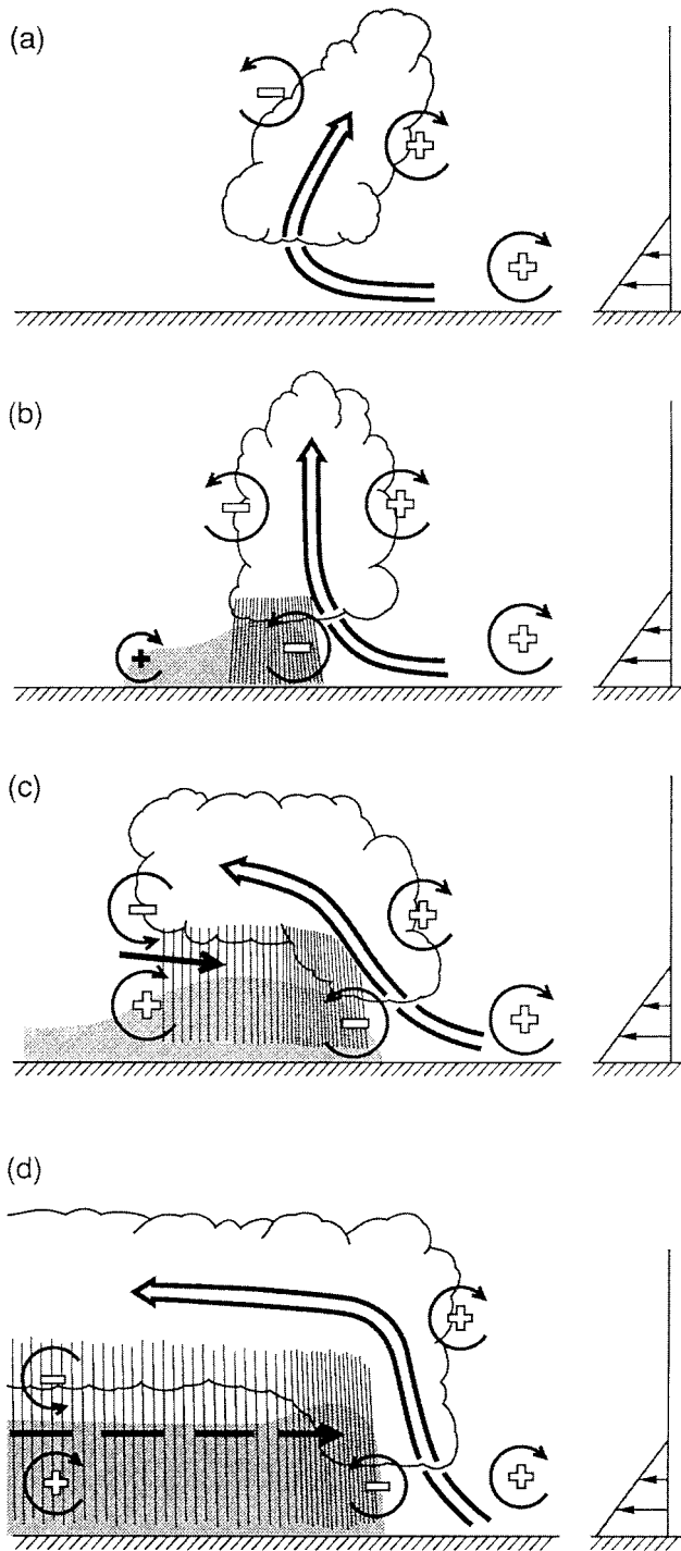
FIG. 23. Four stages in the evolution of an idealized bow echo developing in a strongly sheared, large-CAPE environment. The updraft current is denoted by the thick, double-lined flow vector, with the rear-inflow current in (c) denoted by the thick solid vector. The shading denotes the surface cold pool. The thin, circular arrows depict the most significant sources of horizontal vorticity, which are either associated with the ambient shear or which are generated within the convective system, as described in the text. Regions of lighter or heavier rainfall are indicated by the more sparsely or densely packed vertical lines, respectively. The scalloped line denotes the outline of the cloud. [From Weisman (1993).]
