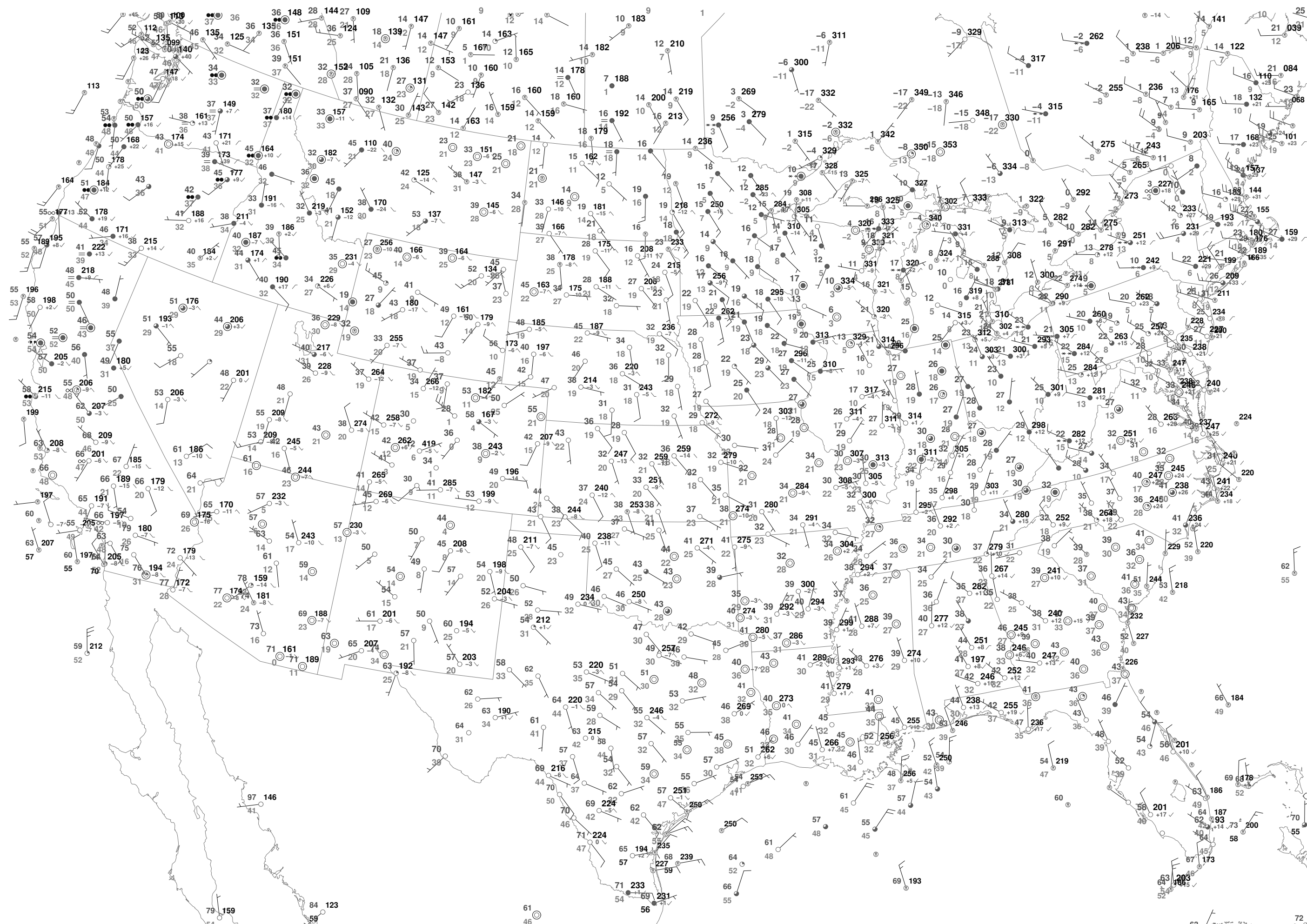
SPC US SFCMAP SUN 241222/0000
