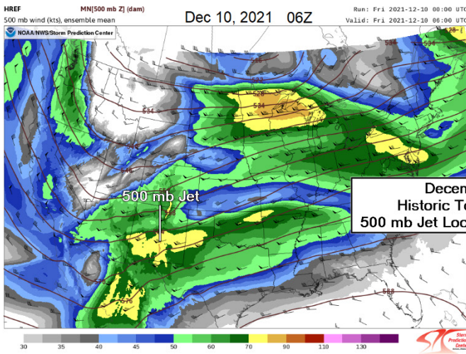
Figure 13. For December 10, 2021, the 500 mb jet's starting location at 06Z (left) and ending location at 00Z (right). The 500 mb jet translation speed for this historic tornado outbreak was 47.3 knots using the 00Z HREF from the evening before the event.
