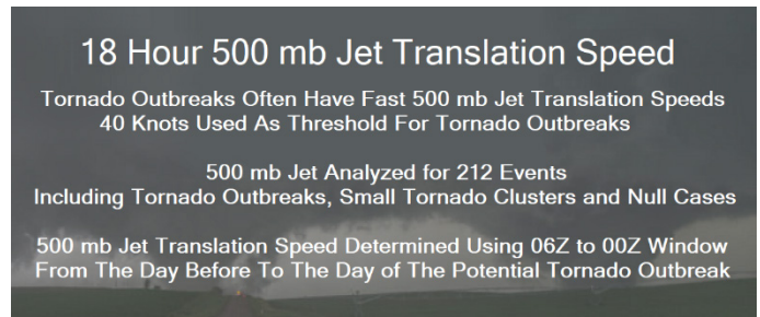
Figure 10. Results of the 500 mb jet translation speed database (212 events) confirm that 40 knots is a good threshold to use to discriminate high-end tornado outbreaks from lower-end ones. To do the analysis, the 500 mb jet translation speed was calculated using an 18 hour window between 06Z the night before and 00Z on the day of the event.
