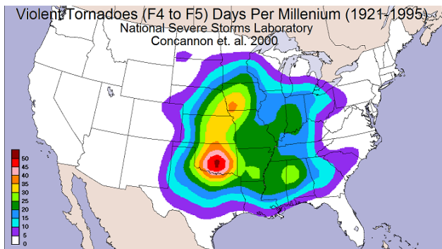
Figure 1. Map of F4 and F5 tornadoes (1921 to 1995) taken from Concannon et al. (2000). A maximum of incidence is noted in the Great Plains. Another maximum is located in the Southeast with a small one in the lower Ohio Valley. The greatest incidence is in the Southern Plains across central and southern Oklahoma.
