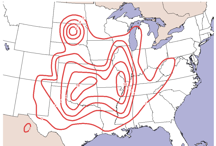
500 mb Jet
