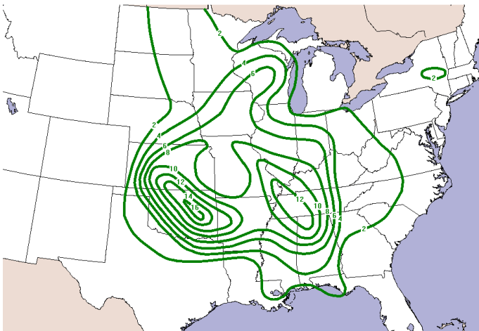
700 mb Jet
