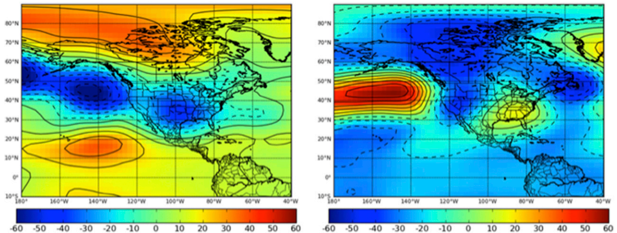
FIG. 19. Monthly anomalies of 500-hPa geopotential height during April (left) El Niño and (right) La Niña conditions.
