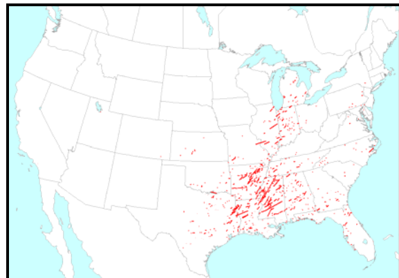
Figure 2a: Tornadoes occurring on "tornado days" during the winter LN phase.
