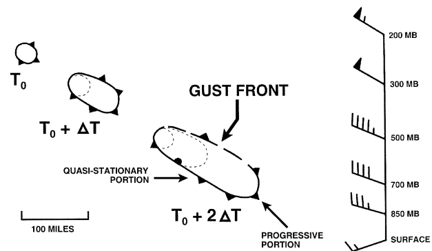
FIG. 2. Plan-view schematic depicting temporal elongation of a cold pool and gust front associated with the hypothetical quasi-unidirectional wind profile shown at right. Motion of boundary relative to ground is depicted by conventional frontal symbols. Dashed lines indicate gust-front positions at earlier times. Indicated spatial scale is for illustrative purposes only.
