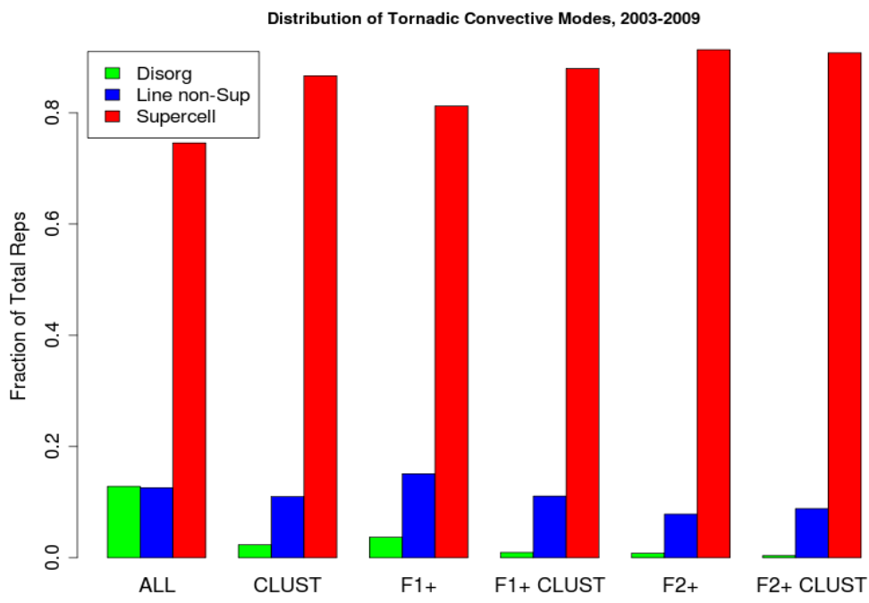
Fig. 18. Fraction of tornado reports by convective mode for each cluster category. ALL = all tornado reports, CLUST = clustered tornado reports, F1+ = all F1+ tornado reports, F1+ CLUST = clustered F1+ tornado reports, F2+ = all F2+ tornado reports, F2+ CLUST = clustered F2+ tornado reports. Green indicates disorganized mode, blue indicates linear non-supercell storm mode, and red indicates supercellular storm mode.
