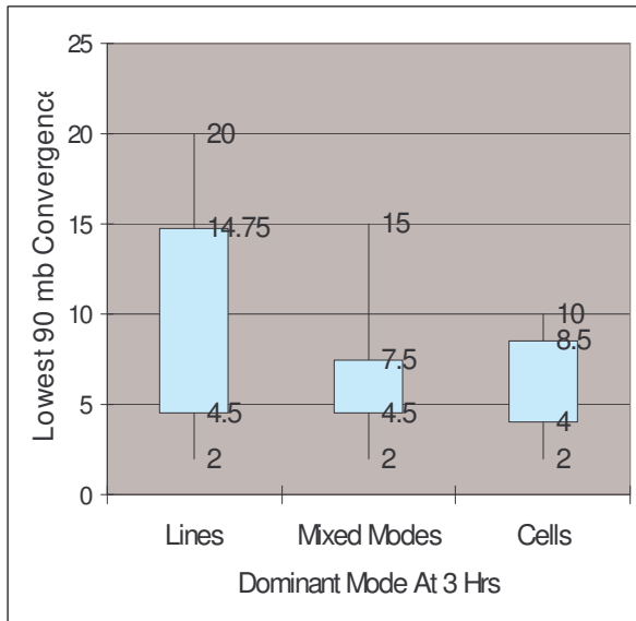
Figure 5. Same as fig. 4 except for low level convergence \times 10^{-5} \text{s}^{-1} .
