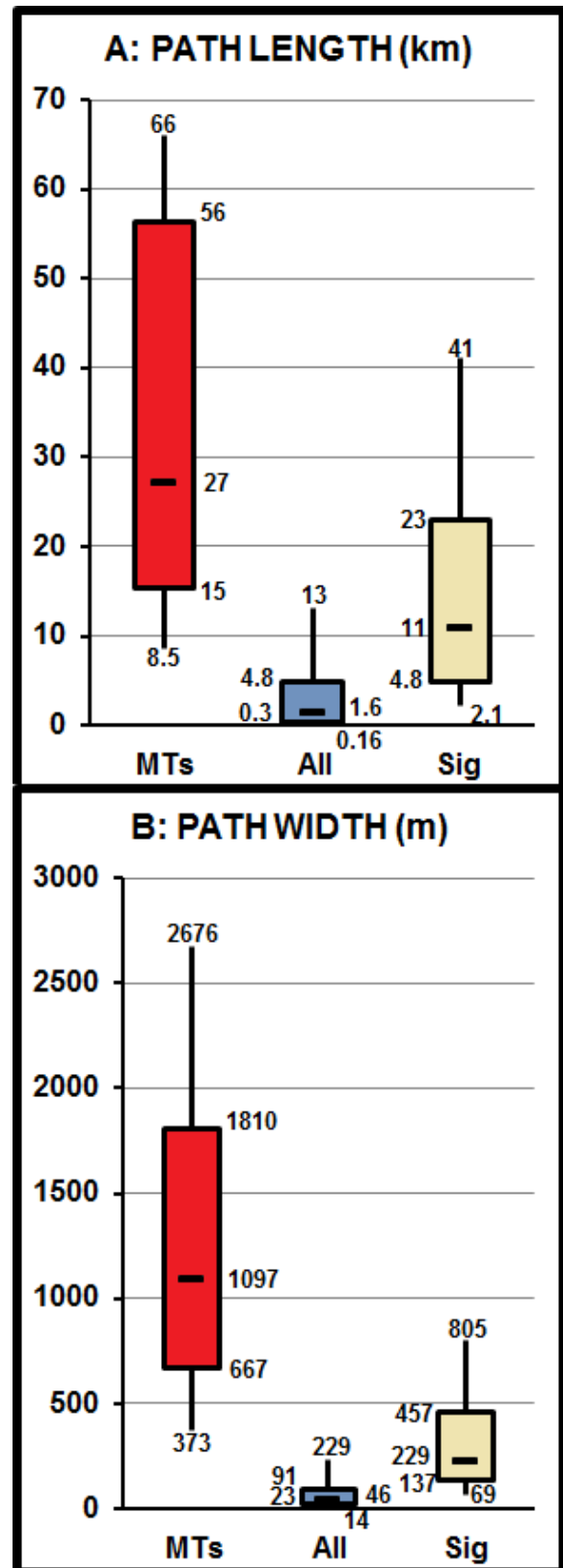
Figure 6: Box-and-whisker diagrams of 1995–2013 distributions of ST-associated MTs, all tornadoes, and significant (Sig, EF2–EF5) tornadoes by a) path length and b) path width as labeled. Boxes represent 25 th –75 th percentiles and whiskers extend to 10 th and 90 th percentiles. Sample sizes: MTs = 23; All = 23 865; Sig = 2628.
