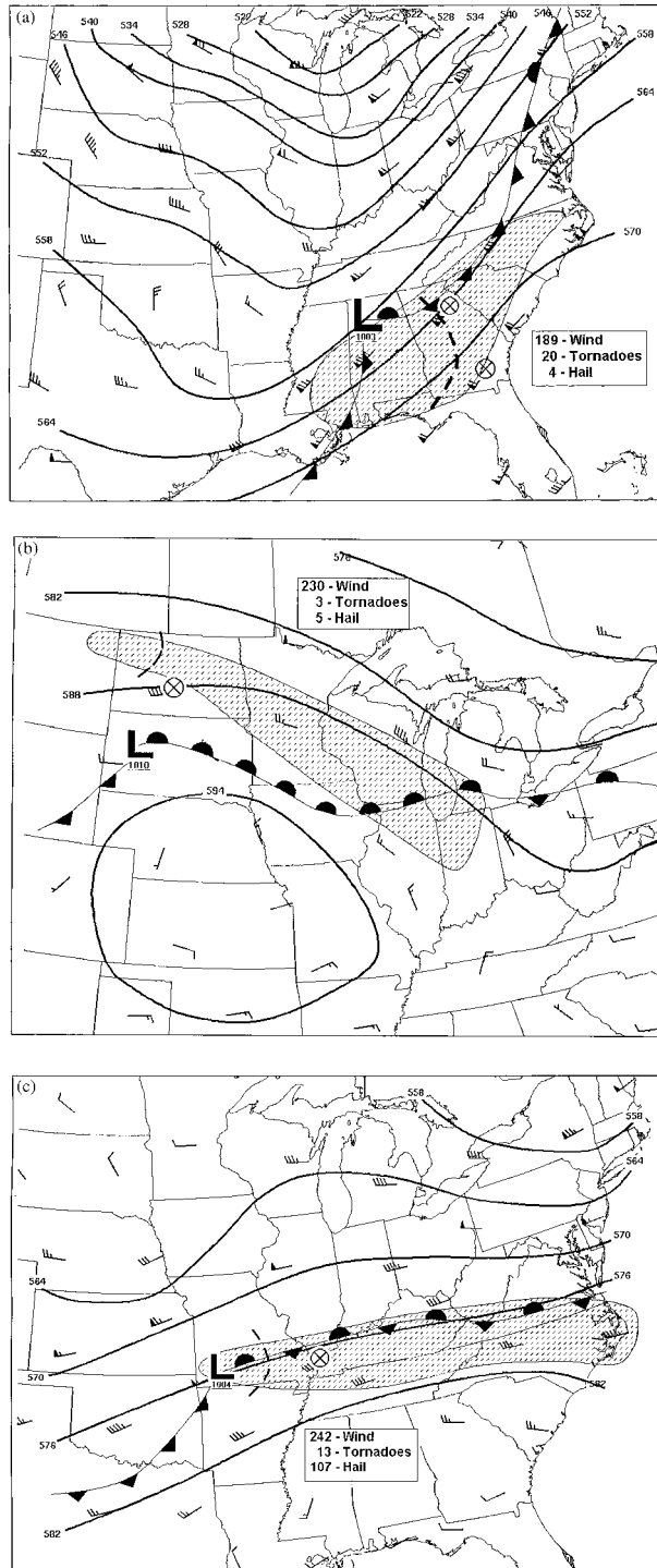
FIG. 1. Examples of the three derecho categories used in this paper. Solid lines depict 500-mb height contours, with the surface low center and frontal locations overlaid. Wind bars are 500-mb winds. All data are at 1200 UTC, the morning prior to the derecho. Hatched area depicts the ensuing derecho's path, with the number of severe reports listed in the box. Dashed line represents the location of the derecho at 1200 UTC, with proximity sounding locations denoted by the \times within a circle: (a) SF derecho on 10 Feb 1990, (b) WF derecho on 19 Jul 1983, and (c) hybrid derecho on 4 Jun 1993.
