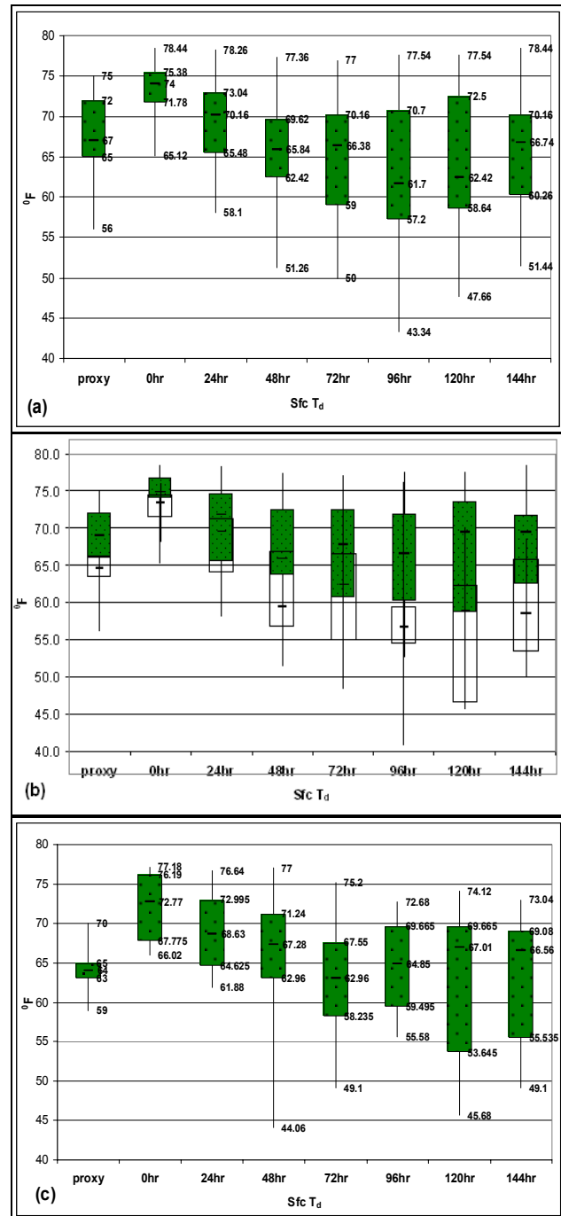
Fig. 2. Event proximity and 0hr buoy 42002 T_d on left, with buoy T_d ( ^\circ F) increasing by 24hr from left to right. Each box and whisker indicates maximum and minimum on either end of line, along with middle 50% values and median within box. a) all SIGTOR, b) SIGTOR separated by months. Oct/Nov color, Dec-Feb clear boxes, c) all SVR.
