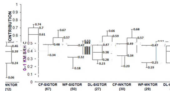
Figure 12: As in Fig. 6, except for the fractional contribution of 0–1-km SRH to the STP.
