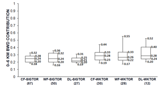
Figure 10: As in Fig. 6, except for the fractional contribution of 0–6-km BWD to the STP.
