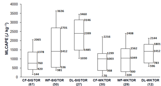
Figure 7: As in Fig. 6, except for MLCAPE (J kg -1 ).
