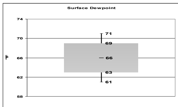
Fig. 6. Box and whiskers diagram of surface dewpoints (°F) observed with cool season Gulf Coast F2+ tornadoes. Box representative of the 25 th and 75 th percentiles, with the outer whiskers representing the 10 th and 90 th percentiles of events.
