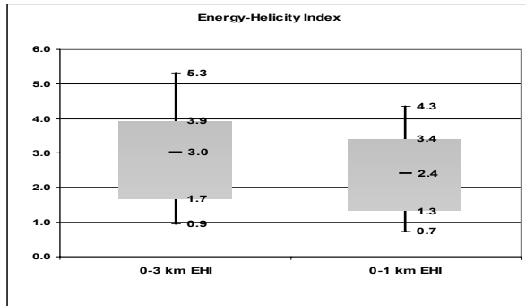
Fig. 14. Same as Fig. 6, except 0-3 km (left) and 0-1 km (right) Energy-Helicity Index (EHI).
