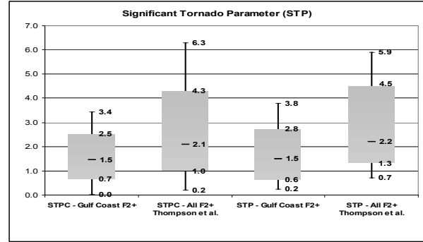
Fig. 16. Same as Fig. 6, except Significant Tornado Parameter (STP) of Gulf Coast F2+ tornadoes vs. a more diverse F2+ tornado dataset by Thompson et al. (2003, 2004, updated 2006). Left half, using the effective layer with CIN (STPC - Thompson et al. 2004). Right, original STP using a fixed layer and no CIN (Thompson et al. 2003).
