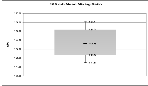
Fig. 8. Same as Fig. 6, except 100 mb mean mixing ratio (g/kg).
