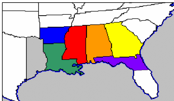
Fig. 1. Map of study domain.
