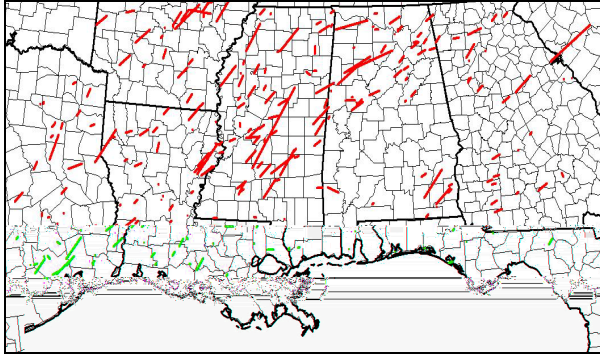
Fig. 2. Map of all F2-F5 tornadoes (with tracks denoted via red lines) between October 15-February 15 from 1984-1985 to 2003-2004.
