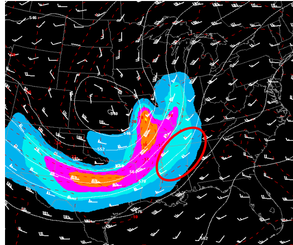
Fig. 4. NARR 500 mb analysis for 12 UTC 24 November 2001. Geopotential heights (standard convention) with wind barbs and shading (beginning at 50 kt with graduated colors every 10 knots) and temperatures (°C) in dashed red. Red oval denotes approximate location of 14 F2+ tornadoes on 24 November 2001.
