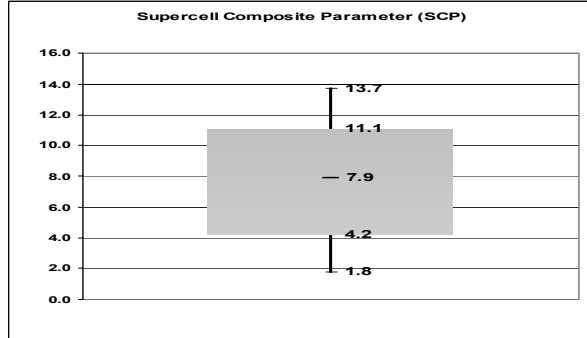
Fig. 15. Same as Fig. 6, except Supercell Composite Parameter (SCP).
