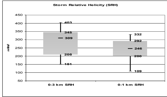
Fig. 13. Same as Fig. 6, except 0-3 km (left) and 0-1 km (right) Storm Relative Helicity (SRH - m^2/s^2 ).
