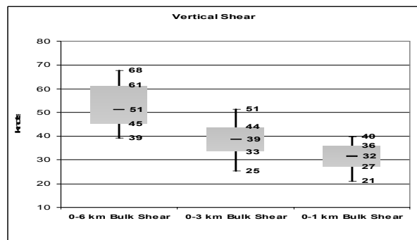
Fig. 12. Same as Fig. 6, except 0-6 km bulk shear, 0-3 km bulk shear, and 0-1 km bulk shear (kt).
