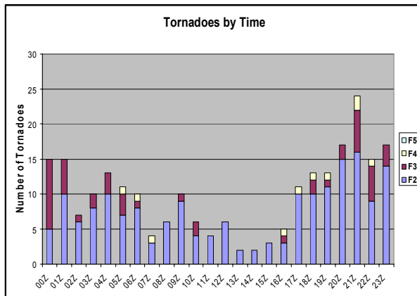
Fig. 3. Cool season Gulf Coast F2-F5 tornadoes by hour (UTC) for October 15-February 15 from 1984-1985 to 2003-2004.
