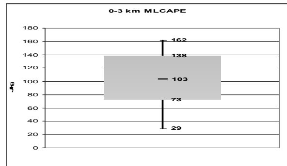
Fig. 11. Same as Fig. 6, except 0-3 km MLCAPE (J/kg).
