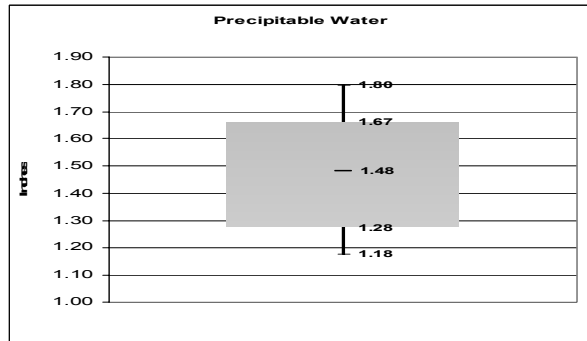
Fig. 9. Same as Fig. 6, except precipitable water (inches).
