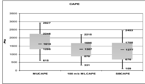
Fig. 10. Same as Fig. 6, except for Most Unstable (MU) CAPE, 100 mb mixed layer (ML) CAPE, and Surface Based (SB) CAPE (J/kg).
