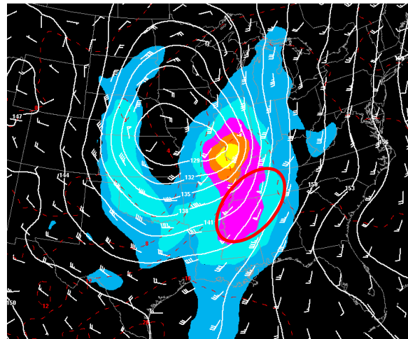
Fig. 5. NARR 850 mb analysis for 12 UTC 24 November 2001. Geopotential heights (standard convention) with wind barbs and shading (beginning at 30 kt with graduated colors every 10 knots) and temperatures (°C) in dashed red. Red oval denotes approximate location of 14 F2+ tornadoes on 24 November 2001.
