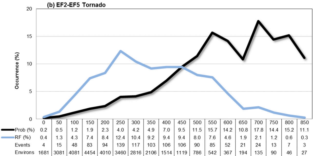
FIG. 10. The Prob (black) and RF (blue) plots for effective SRH ( m^2 s^{-2} ) corresponding to (a) weak and (b) significant tornado events. These plots use constraints for organized, surface-based convection: effective bulk shear at least 50 kt, MLCAPE at least 1000 J kg^{-1} , MLCIN less negative than or equal to -50 J kg^{-1} , and MLLCL at or below 1500 m.
