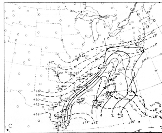
FIGURE 5.—850-mb. charts for February 1, 1955, showing isotherms (dashed) and dew point lines (solid) for 2^{\circ} C. intervals at (A) 0900 cst, (B) 1500 cst, and (C) 2100 cst.
