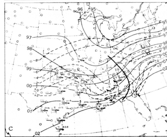
FIGURE 6.—700-mb. charts for February 1, 1955, showing contours (light solid lines) for 100-ft. intervals, isotherms (dashed lines) for 2^{\circ} C. intervals and the "no-change" line (heavy solid line) at (A) 0900 cst, (B) 1500 cst, and (C) 2100 cst.
