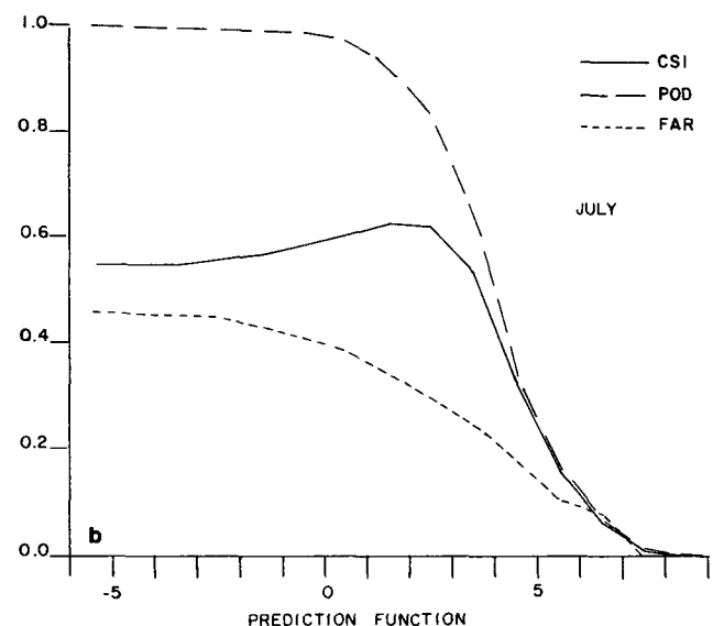
FIG. 2b. As in Fig. 2a except during July as a function of J1.
