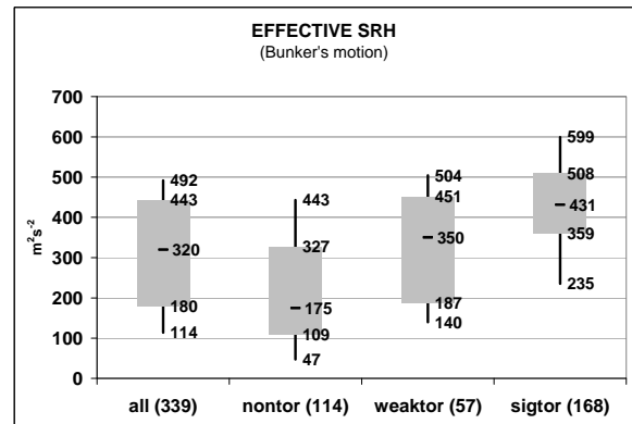
Fig. 21 Box and whiskers plot (same conventions as in Fig 18) except for Effective SRH ( m^2s^{-2} ) estimated via the Bunker's et al. (2000) storm motion algorithm for all four storm groups.
