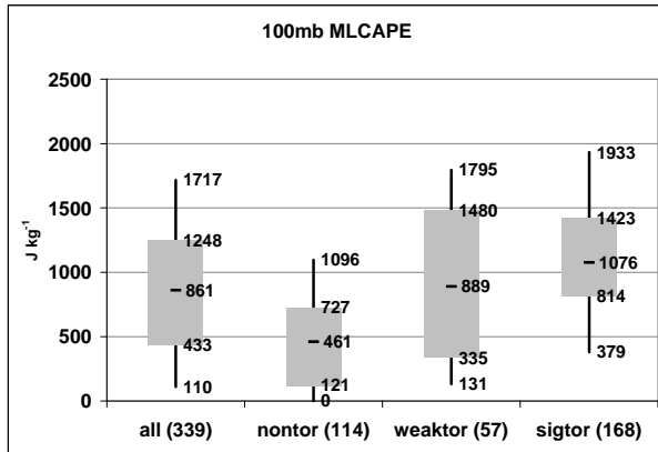
Fig. 18 Box and whiskers plot of MLCAPE ( J kg^{-1} ) for supercell grid hours for all supercells (339), non-tornadic supercells (nontor, 114), weakly tornadic supercells (weaktor, 57) and significantly tornadic supercells (sigtor, 168). The shaded box covers the 25 th -75 th percentiles, the whiskers extend to the 10 th and 90 th percentiles, and the median values are marked by the heavy horizontal line within each shaded box.
