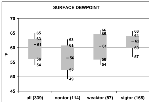
Fig. 19 Same as in Fig 18 except for surface dewpoint ( ^{\circ}F ).
