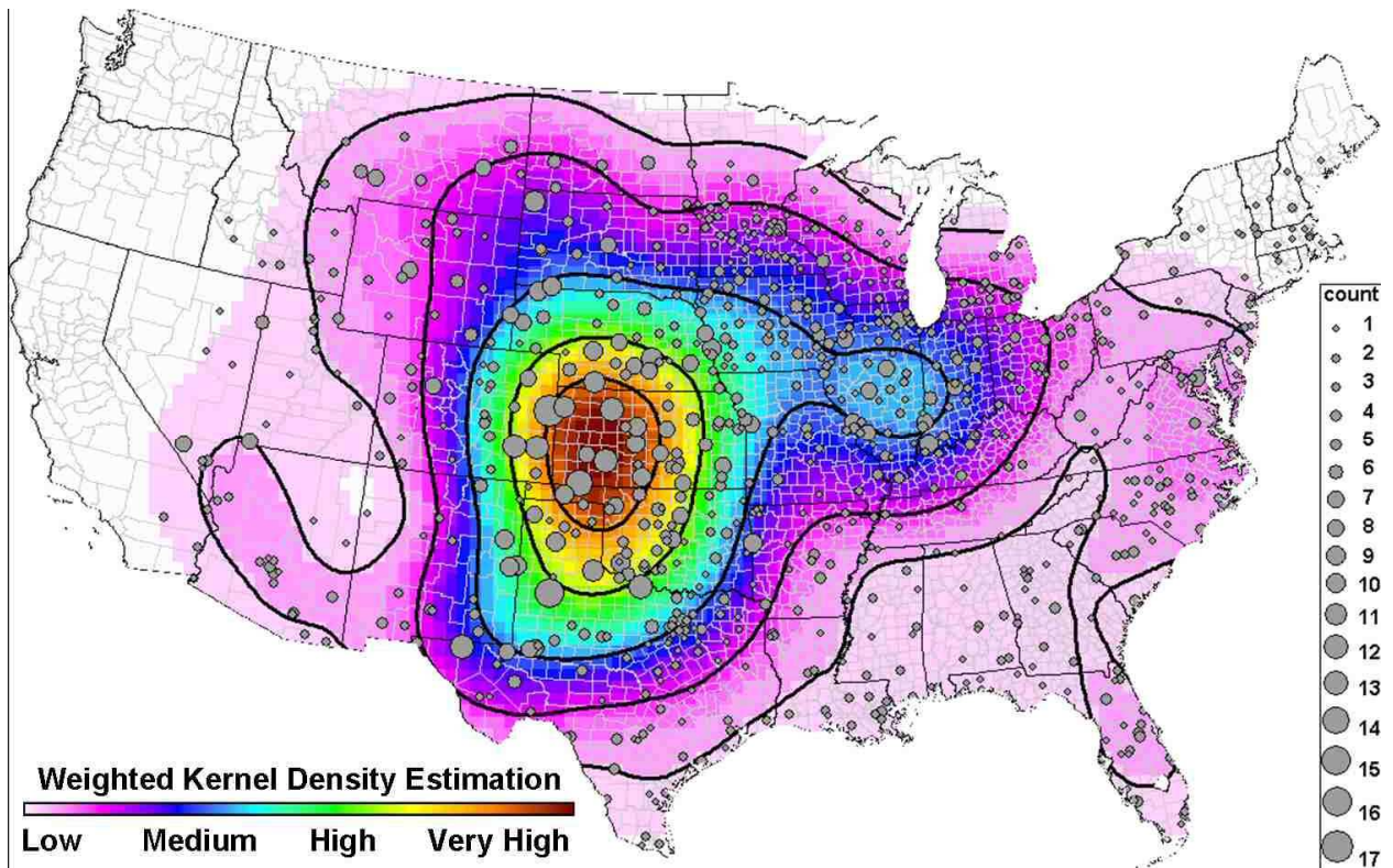
Figure 4. Kernel density estimation plot of ASOS/AWOS stations 2003-2009 that observed \geq 1 severe gust and weighted by wind gust count per station. The outermost black contour contains 90% of the kernel density estimation of events, with subsequent 75%, 50%, 25%, and 10% contours inward. Proportional symbol plot of stations' counts that measured 50 \geq kts denoted by gray circles.
