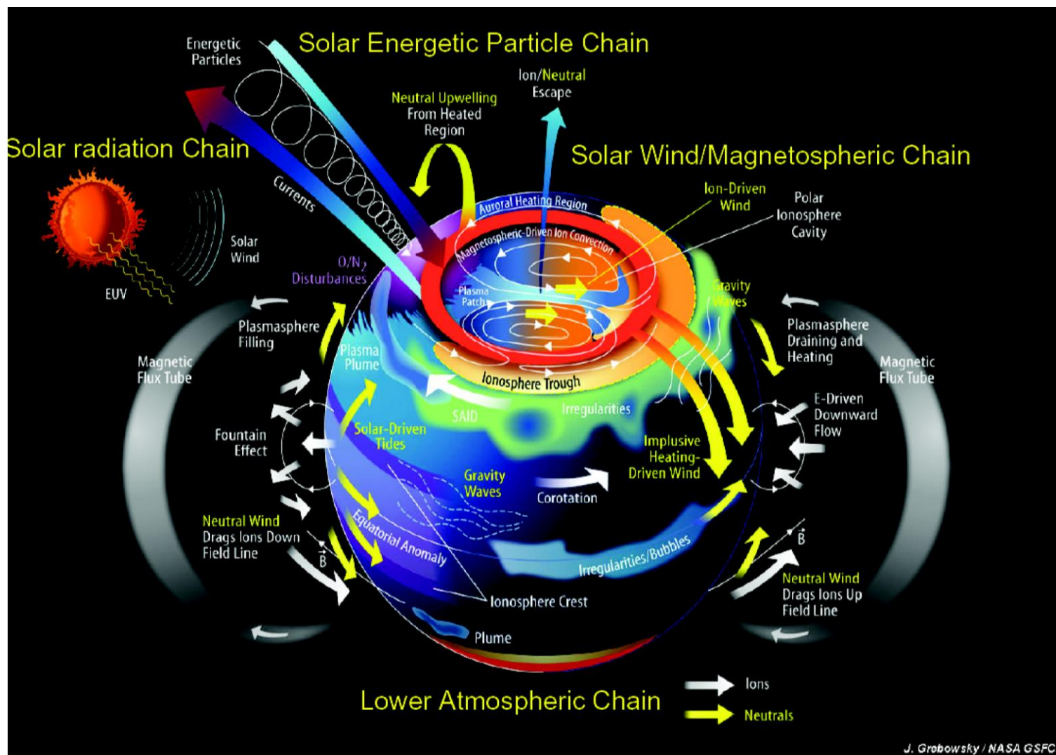
Terrestrial Processes and Sources Impacting Neutral Density
