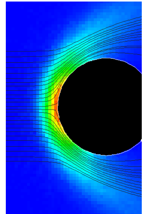
A DSMC simulation for force-coefficient computation
