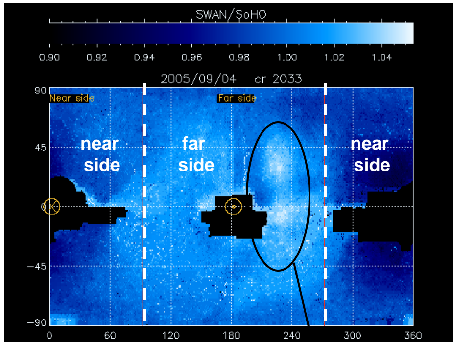
Lyman-alpha radiation far-side back-scattering ( Quemerais, Bertaux et al. )
