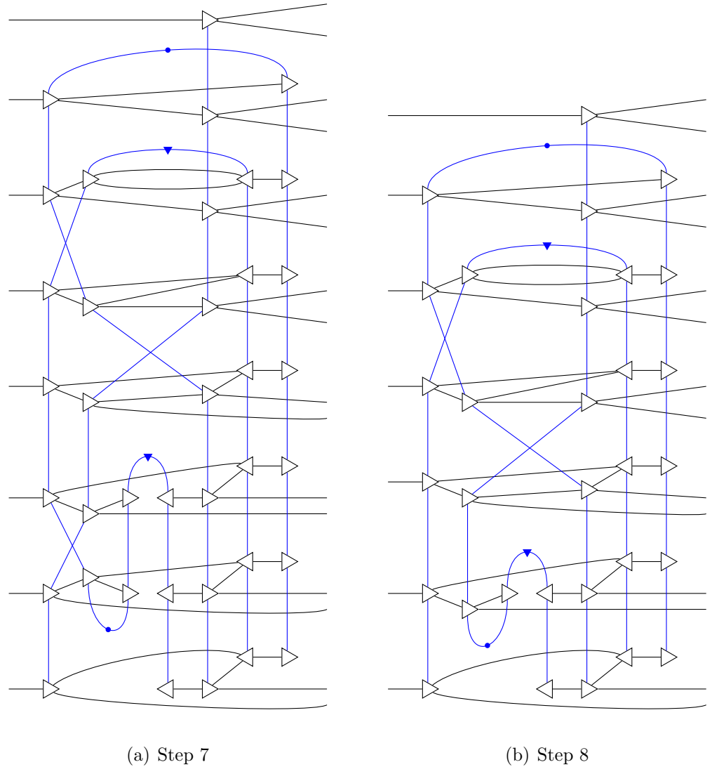
Figure 28: Upper part IV, from the proof of Theorem 6.9(i)
