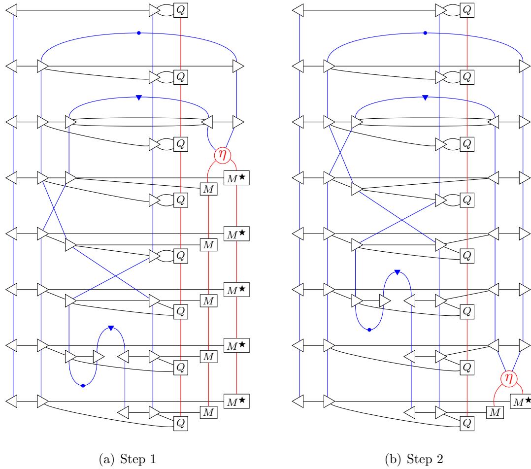
Figure 25: Upper part I, from the proof of Theorem 6.9(i)
