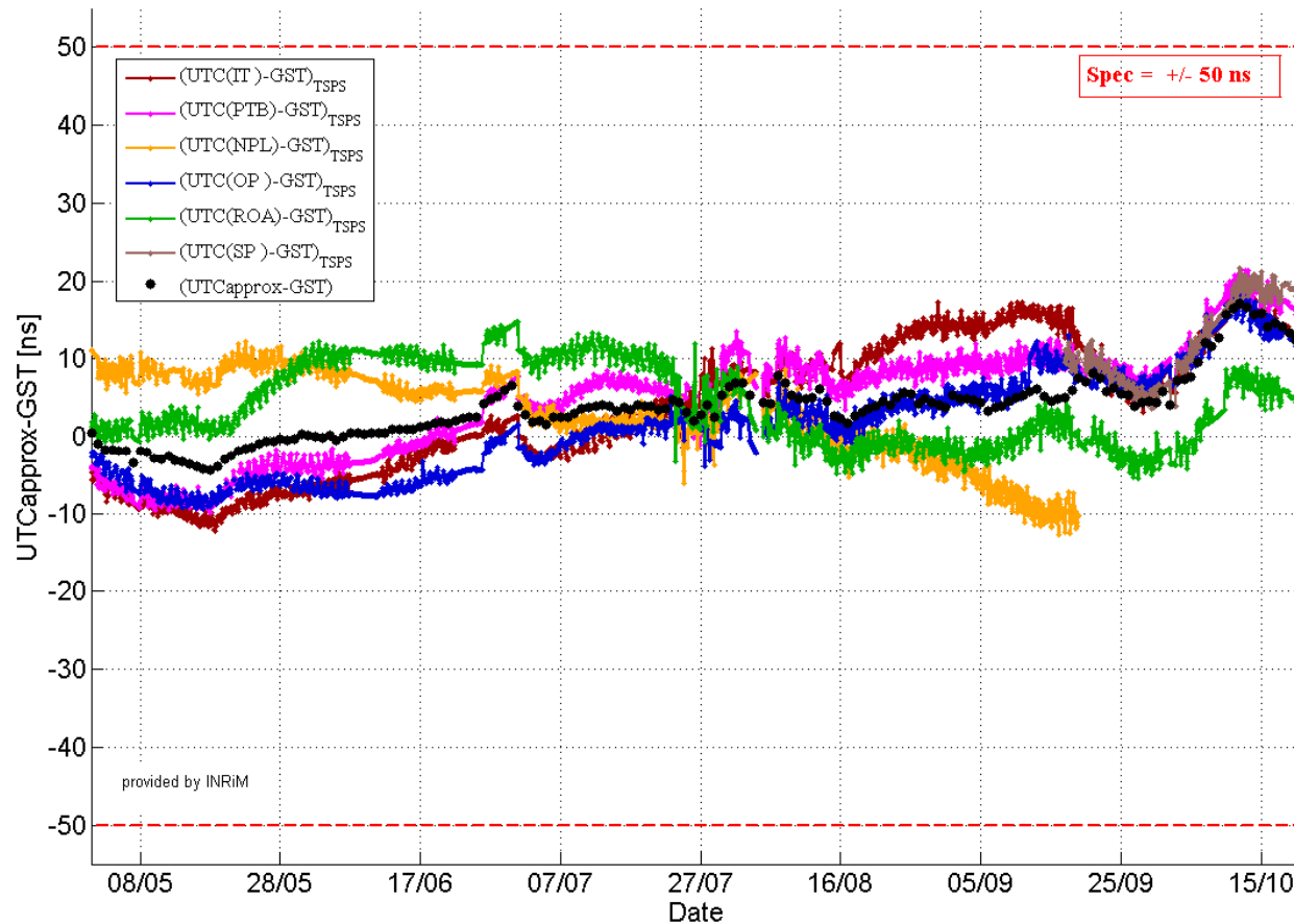
UTCapprox-GST (00 UTC) and TSPS baselines from 01/05/13 to 20/10/13 (MJD 56413 - 56585)
