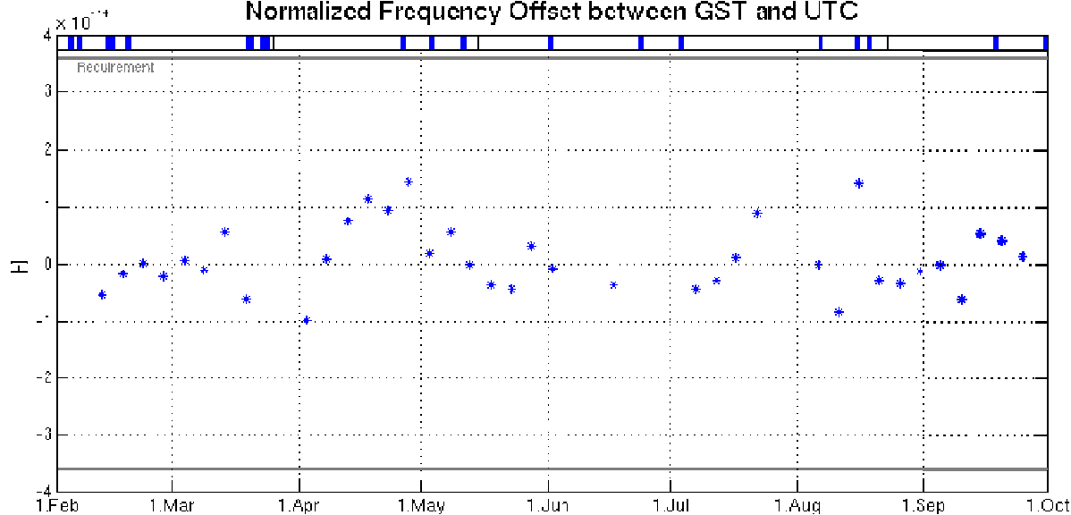
Normalized Frequency Offset between GST and UTC
