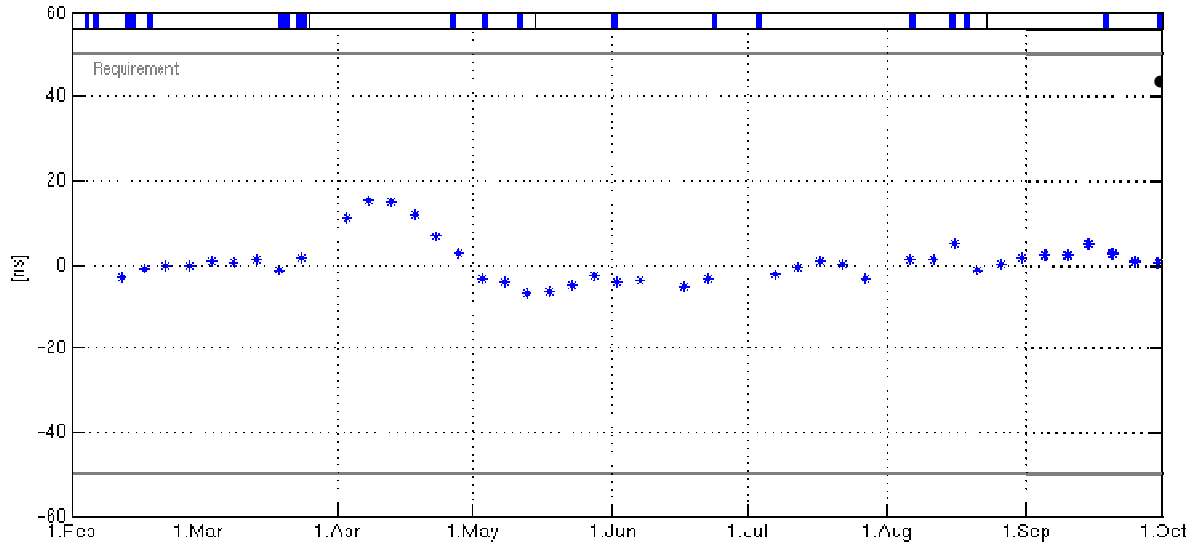
GST vs. UTC Time Offset
