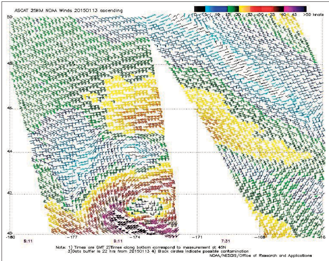
Figure 32. ASCAT (METOP-A) image of satellite-sensed winds (25-km resolution) around the hurricane-force cyclone shown in the second part of Figure 31. The valid time of the pass containing the strongest winds is 0911 UTC January 13, 2015, or about three hours later than the valid time of the second part of Figure 31. Image is courtesy of NOAA/NESDIS/ Center for Satellite Application and Research.
