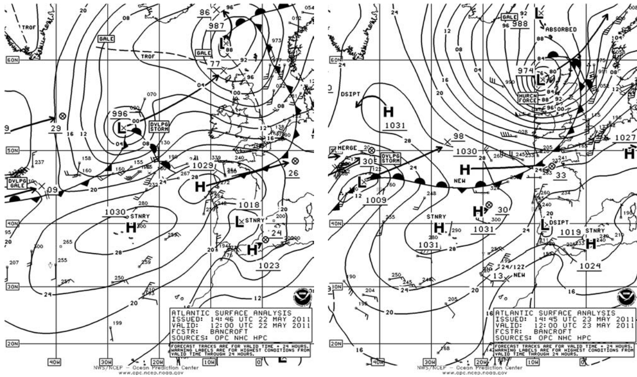
Figure 18. OPC North Atlantic Surface Analysis charts valid 1200 UTC May 22 and 23, 2011.
