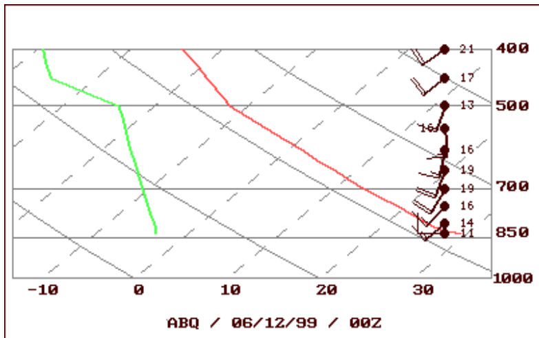
Figure 4. Sounding data (below 400mb) for Albuquerque on June 12, 1999 at 00Z.
