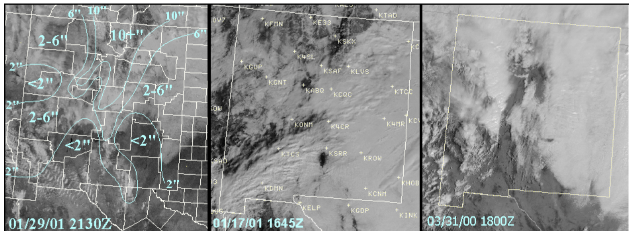
Figure 9. Visible satellite images during or following spill over wind events.
