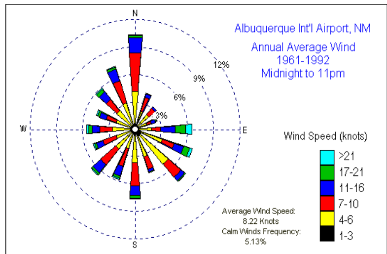
Figure 1. Annual wind rose for Albuquerque for years 1961-1992.
