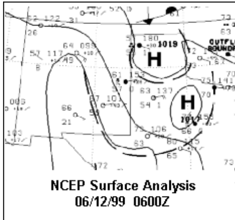
Figure 6. Surface analysis for June 12, 1999 at 0600Z.
