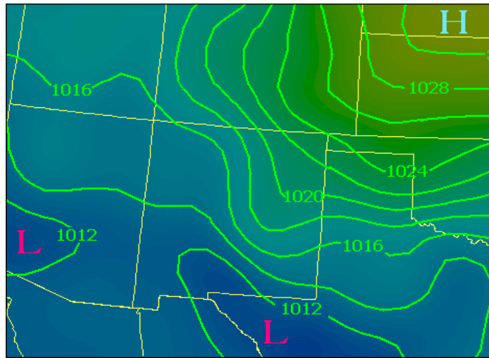
Figure 2. Surface pressure (mb) pattern associated with gap wind events.
