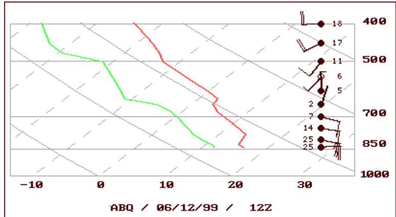
Figure 7. Sounding data (below 400 mb) for Albuquerque on June 12, 1999 at 12Z.
