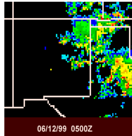
Figure 5. Radar reflectivity mosaic (from NCDC) on June 12, 1999 at 05Z.
