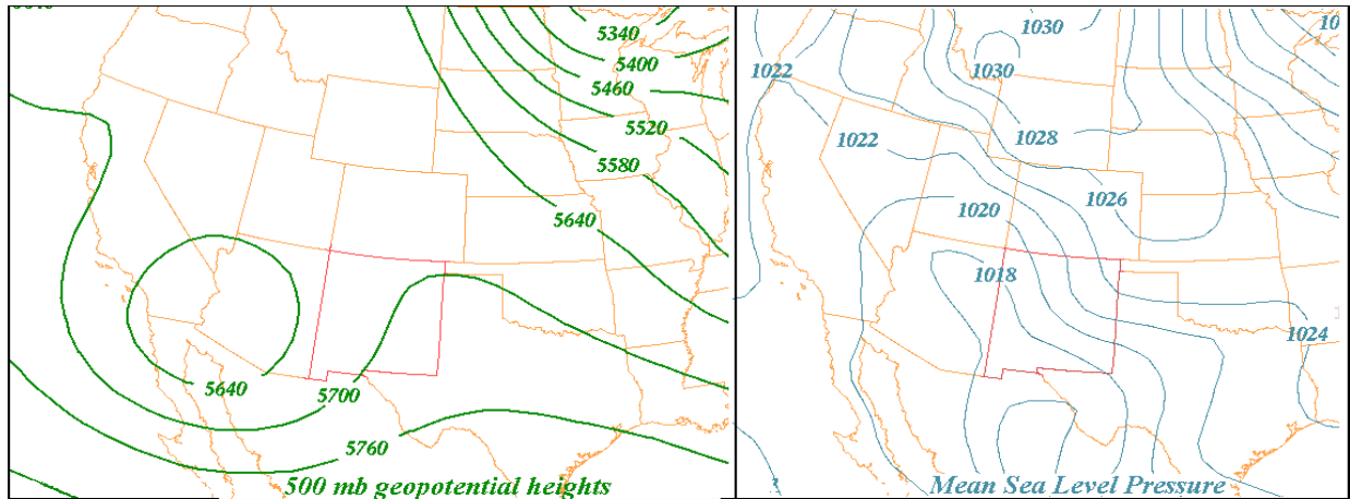
Figure 8. Synoptic pattern for spill over winds with 500 mb heights (left) and mean sea level pressure (right).
