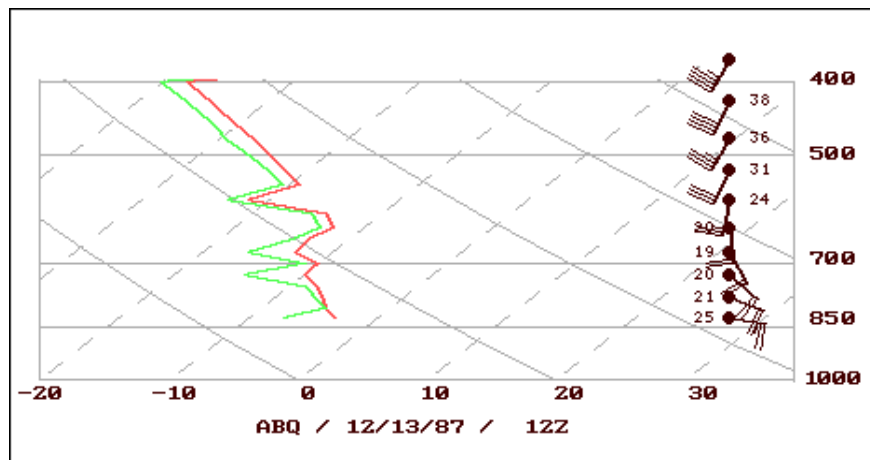
Figure 10. Sounding data (below 400 mb) for 12Z on December 13, 1987.
