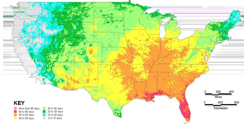
Average Number of Thunderstorm Days per Year
