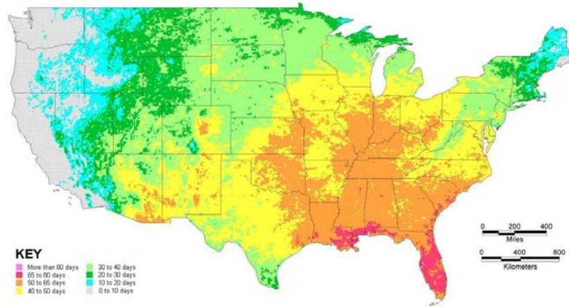
Average Number of Thunderstorm Days per Year
