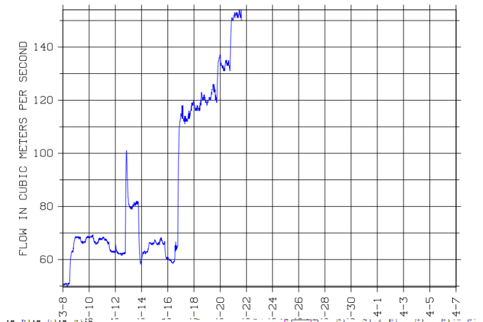
8-4613.00 Rio Grande Below Falcon Dam Falcon TX Data are provisional // Latest Data 3/21/2013 15:15 CST
