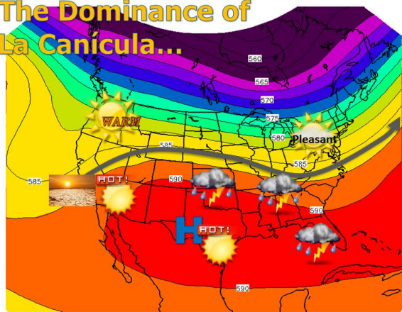
500mb GEOPOTENTIAL HEIGHTS (dam) 51-DAY MEAN FOR: Wed JUL 01 2015 - Thu AUG 20 2015 NCEP OPERATIONAL DATASET
