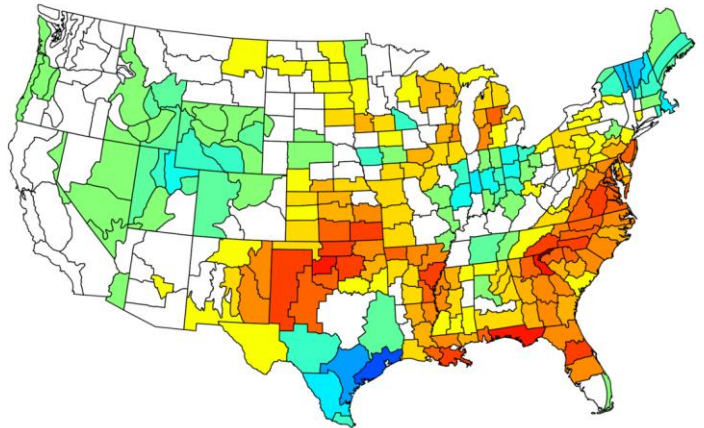
NOAA/NCDC Climate Division Composite Precipitation Anomalies (in) Jun to Aug 1973,1983,1998 Versus 1950-1995 Longterm Average
