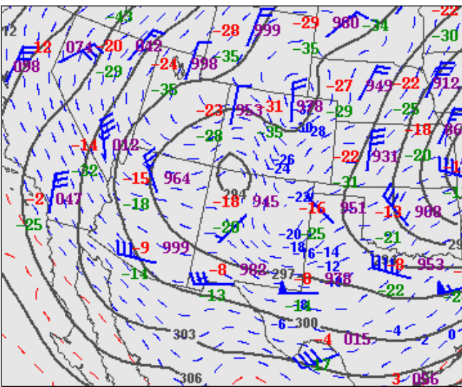
Figure 5 – 700mb Analysis valid 00z 02/02/2011 (5pm MST 02/01/2011), showing upper low over the Four Corners Region.
