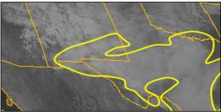
Figure 10 – Visible Satellite Image from 21z (2pm MST) 2/2/2011. Cloudy areas outlined in yellow to distinguish from snow covered ground.
