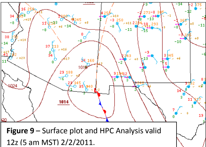
Figure 9 – Surface plot and HPC Analysis valid 12z (5 am MST) 2/2/2011.
