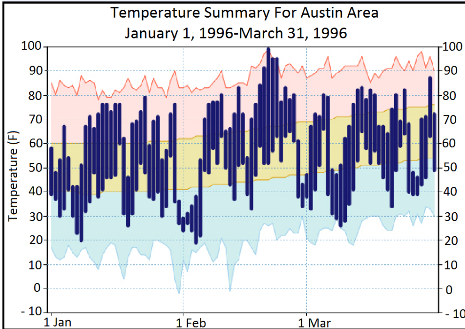
Figure 1. Daily temperature chart for Austin from Jan 1-March 31, 1996. Observed daily maximum and minimum connected by dark blue line. The red line connects record high temperatures, and the blue line connects record low temperatures.
