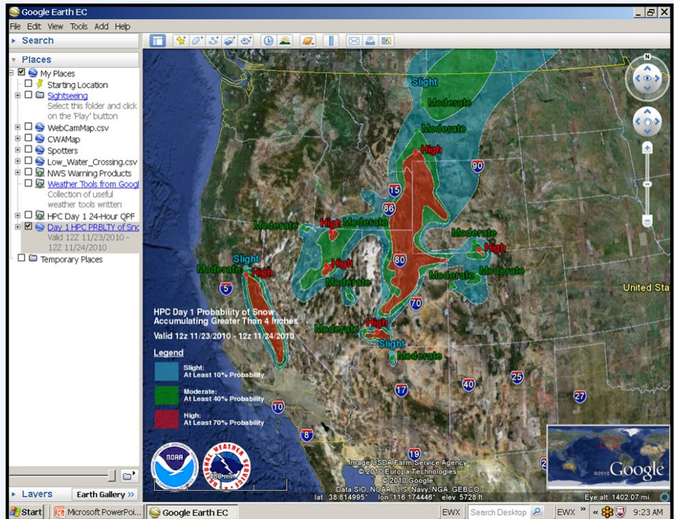
Above: HPC Day 1 Winter Weather Probability displayed in Google Earth.
