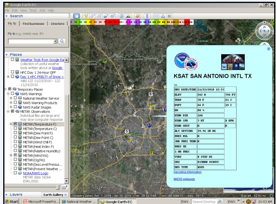
Figure 1: Surface Observations available from the NWS GIS Portal displayed in Google Earth. Available at www.weather.gov/gis
