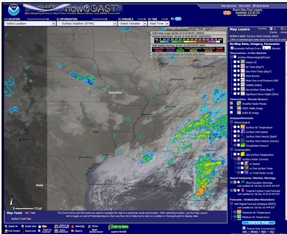
Above: NOAA nowCOAST displaying visible satellite and a radar mosaic.
