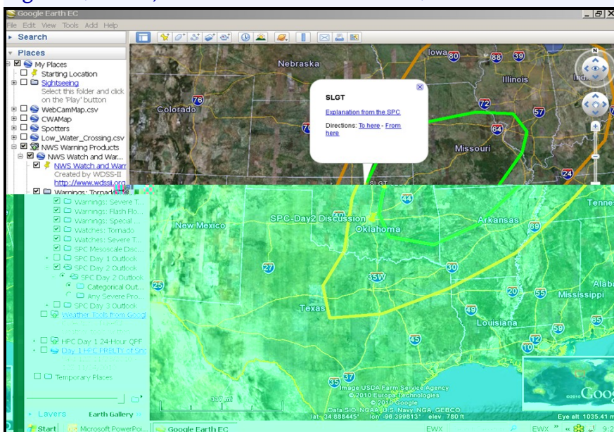
Figure 2: SPC Day 2 Convective Outlook from the NWS GIS Portal displayed in Google Earth.
