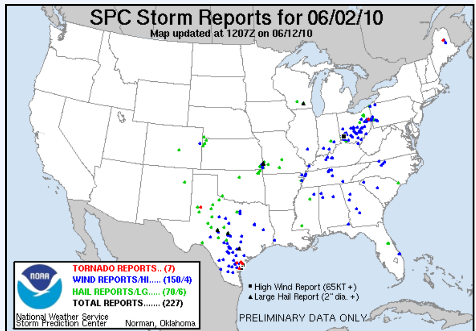
Above: An example of the Storm Prediction Center's Storm Reports plot.
