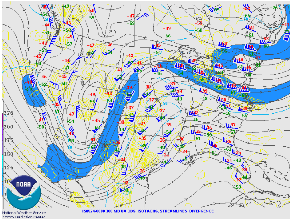
Figure 6: 300mb winds and divergence outlined in yellow. Note the sharp air flow direction change across northern Mexico with a potent long wave trough. This strong diffluence allowed for strong horizontal divergence that supported stronger and long-lived updrafts that tapped into the ample moisture in place over Texas. Note the high contouring of yellow outlines across south central Texas.
