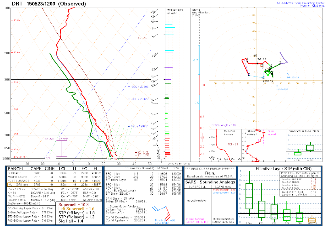
Figure 5: SPC Sounding chart from KDRT 05/23 12Z. Note the PW value of 1.83" taken from the weather balloon sampling in Del Rio, Texas from Saturday morning. CAPE values were already high that morning ahead of developing storms and indicated more storms would be likely that afternoon. This instability in combination with modest shear values allowed for organized storms to develop.
