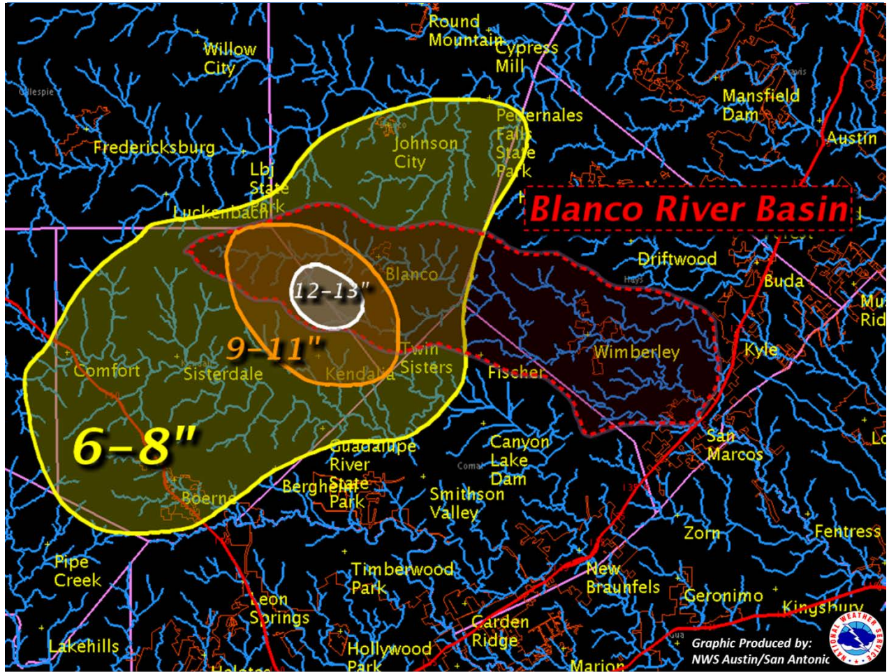
Figure 2: Widespread 6-8 inches of rainfall with local 9 to 11 inches and a maximum of 12-13 inches fell in the head waters of the Blanco River Basin over 4-6 hours.
