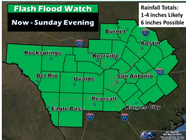
Figure 8: Flash Flood Watch issued at 3:12am
