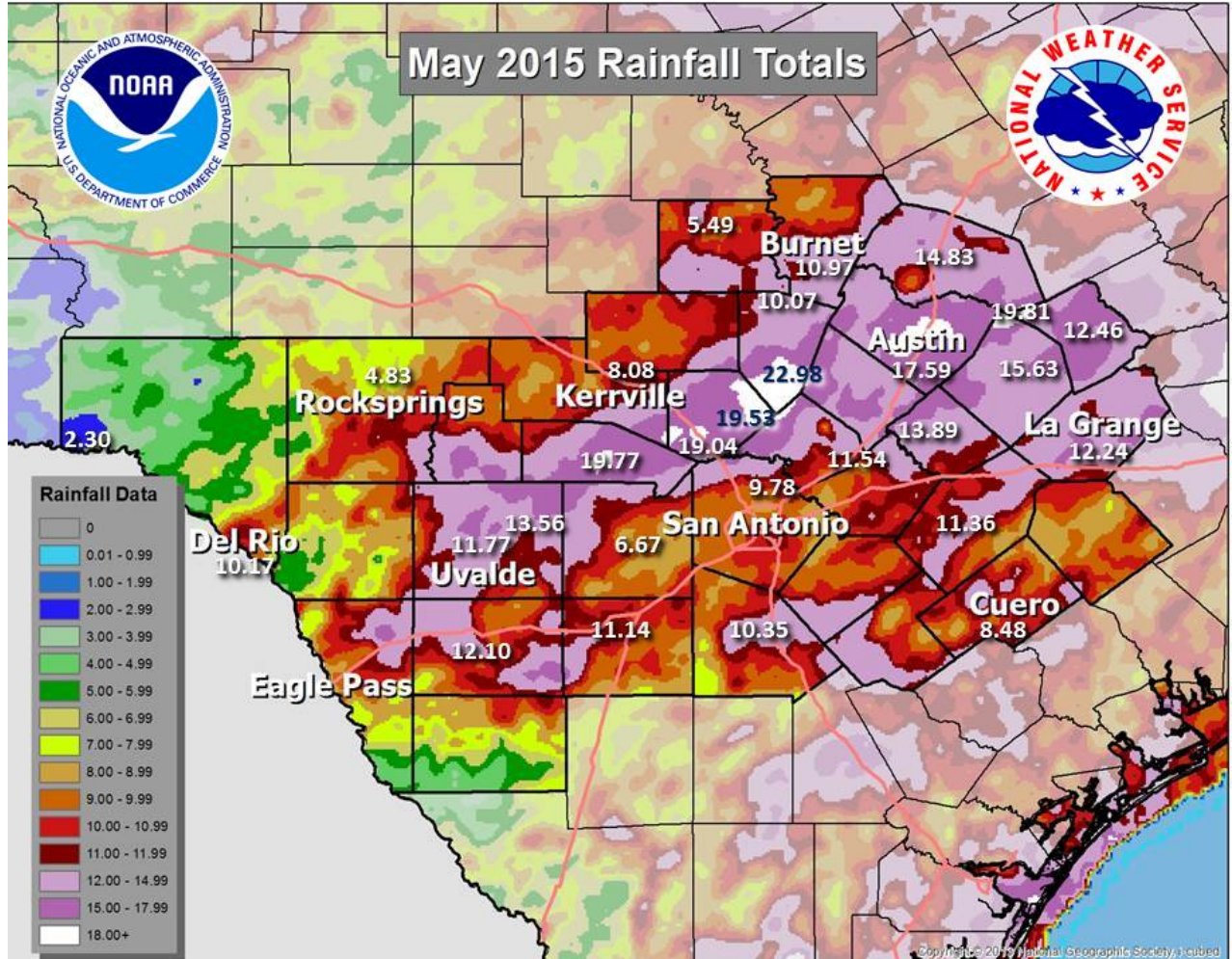
Figure 1: May 2015 rainfall totals.
