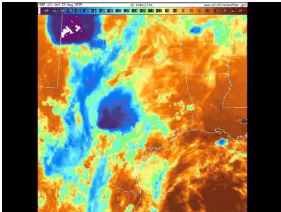
Infrared Satellite loop from May 23, 2015
