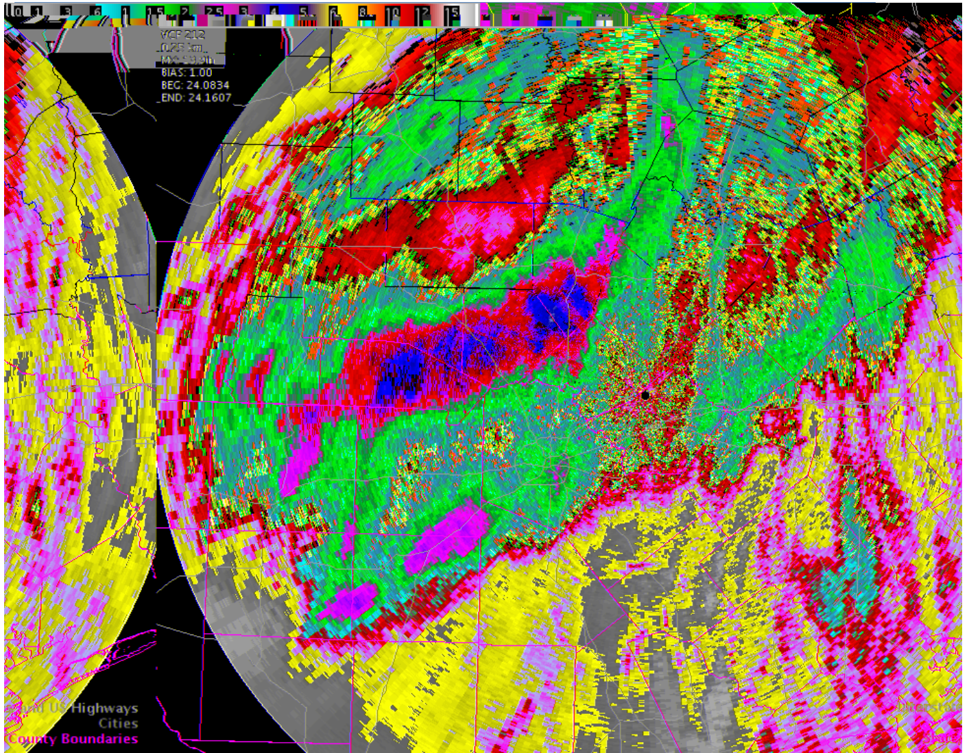
Figure 13: Dual-Polarization Radar Storm total Rainfall Estimates. Note the 9-11 inches with Max nearing 13" in the dark red to White area along the Blanco/Kendall County Line
