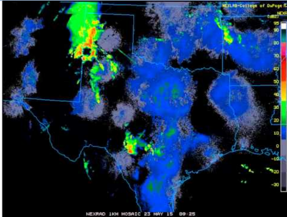
Radar loop from 7pm CDT May 22 – 7pm CDT May 23, 2015
