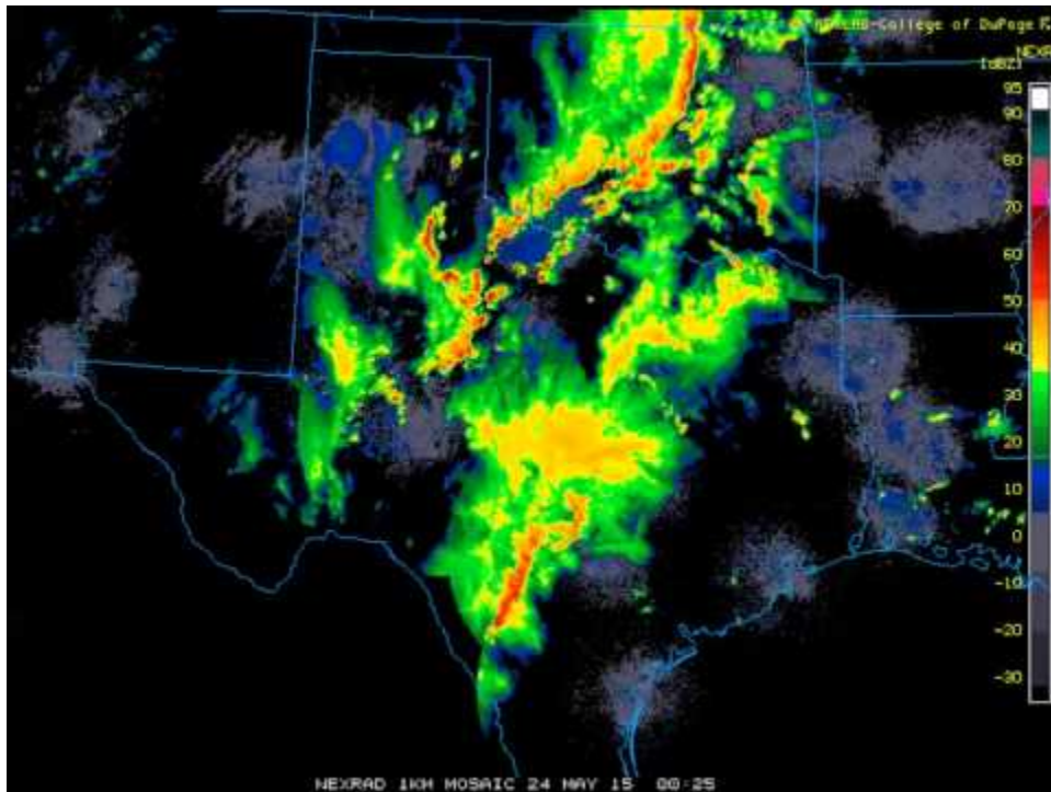
Radar loop from 7pm CDT May 23 – 7pm CDT May 24, 2015
