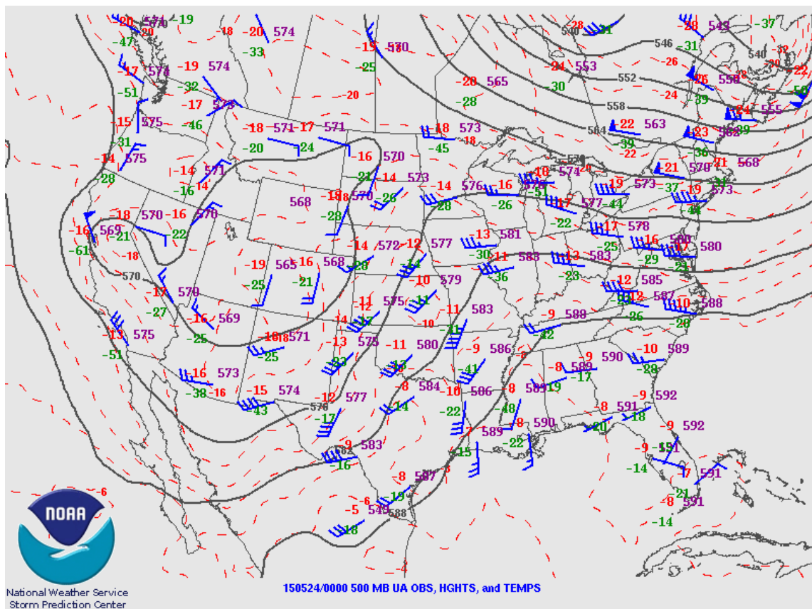
Figure 4: 500 mb chart for 5/24 at 00z (May 23 7pm). Mid-level Atmospheric pattern on May 23rd at 7pm. Note the little ripples in the lines over Texas. These ripples can indicate enhanced areas of lift and when combined with cyclonically-curved winds, can result in supportive environment for longer lived storms.
